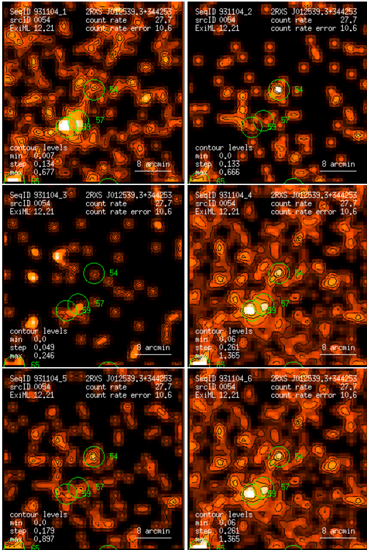
Figure 54: RASS 931104: detection 0054: band rate images, Gaussian filter: (1) PSPC channels 11 – 41, (2) 52 – 90, (3) 91 – 201, (4) 11 – 235, (5) 52 – 201, (6) 11 – 201. Broad band rates in counts/ks. Band rate contour levels in counts/ks/arcmin 2 .
