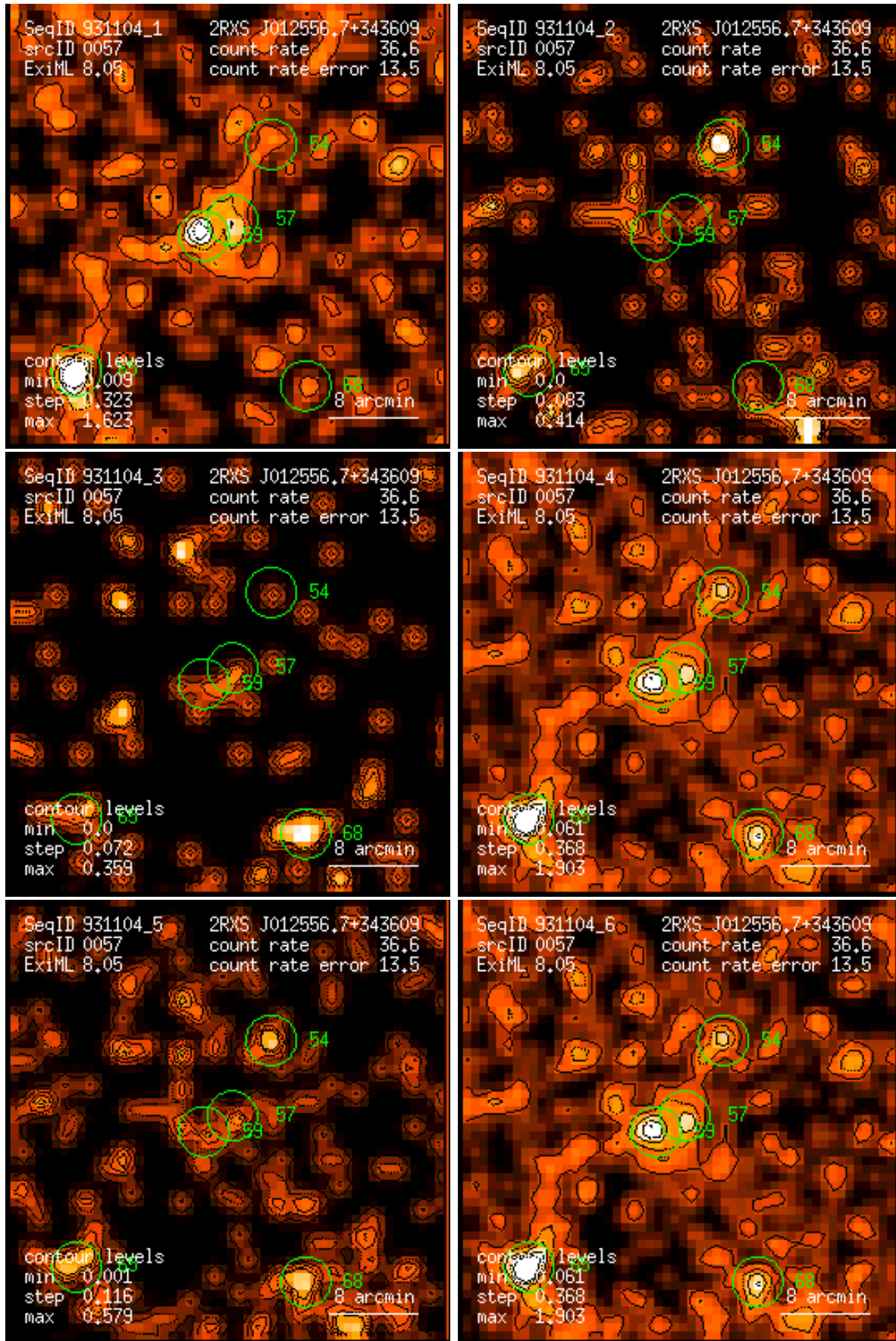
Figure 57: RASS 931104: detection 0057: band rate images, Gaussian filter: (1) PSPC channels 11 – 41, (2) 52 – 90, (3) 91 – 201, (4) 11 – 235, (5) 52 – 201, (6) 11 – 201. Broad band rates in counts/ks. Band rate contour levels in counts/ks/arcmin 2 .
