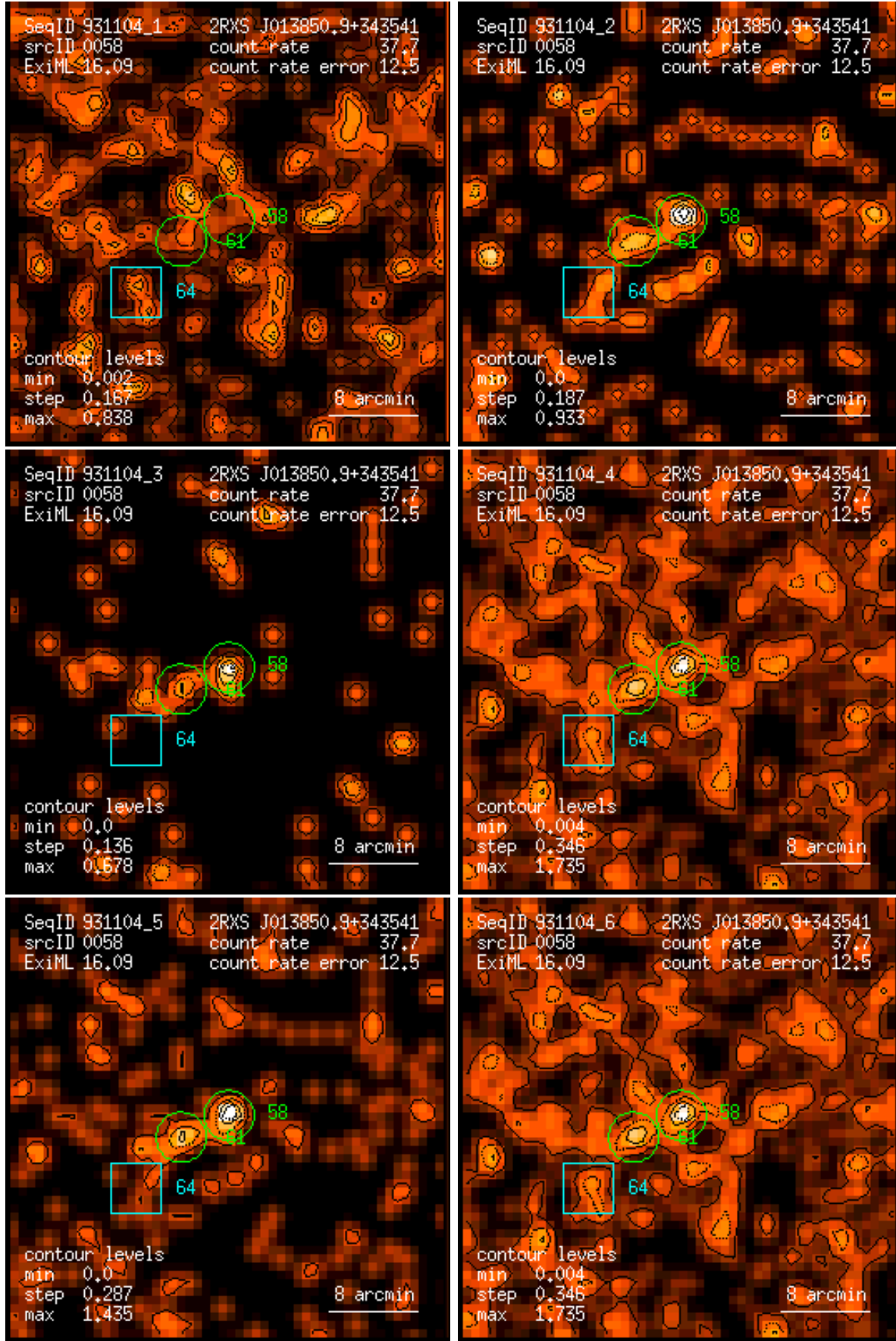
Figure 58: RASS 931104: detection 0058: band rate images, Gaussian filter: (1) PSPC channels 11 – 41, (2) 52 – 90, (3) 91 – 201, (4) 11 – 235, (5) 52 – 201, (6) 11 – 201. Broad band rates in counts/ks. Band rate contour levels in counts/ks/arcmin 2 .
