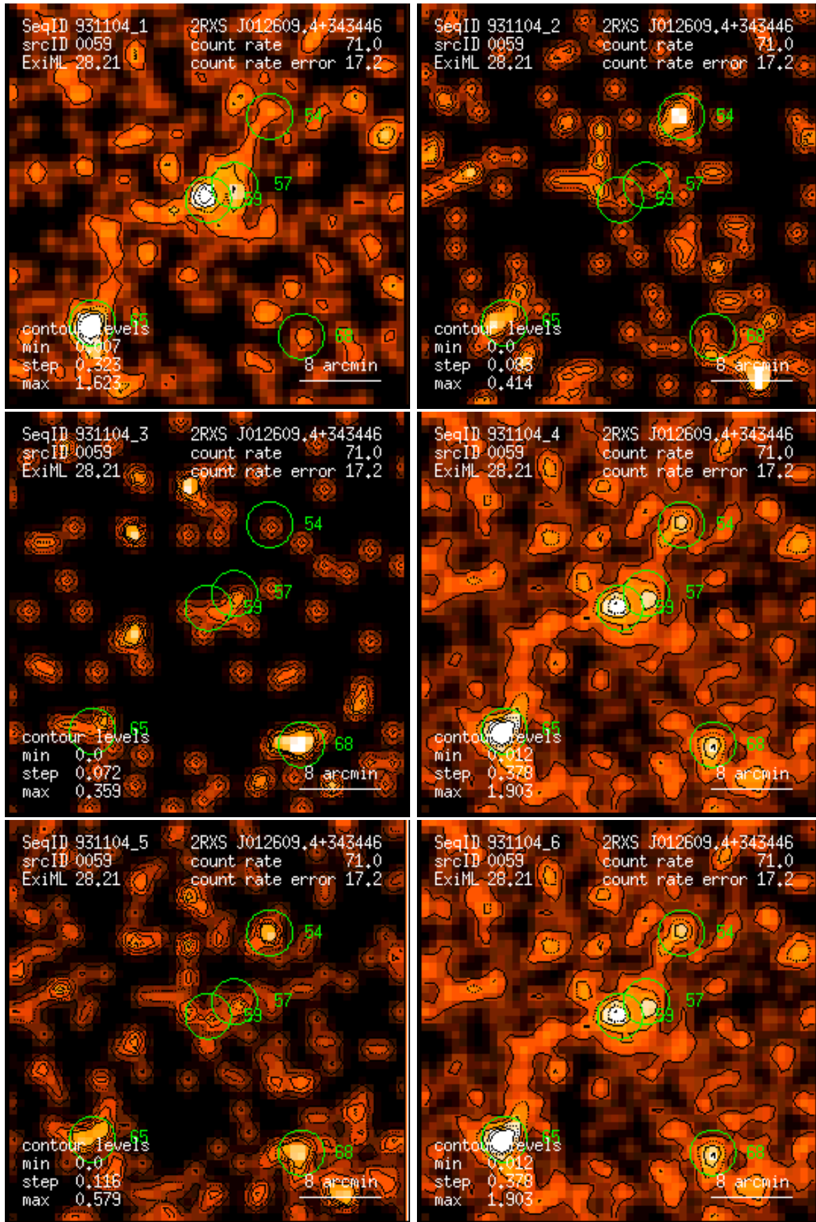
Figure 59: RASS 931104: detection 0059: band rate images, Gaussian filter: (1) PSPC channels 11 – 41, (2) 52 – 90, (3) 91 – 201, (4) 11 – 235, (5) 52 – 201, (6) 11 – 201. Broad band rates in counts/ks. Band rate contour levels in counts/ks/arcmin 2 .
