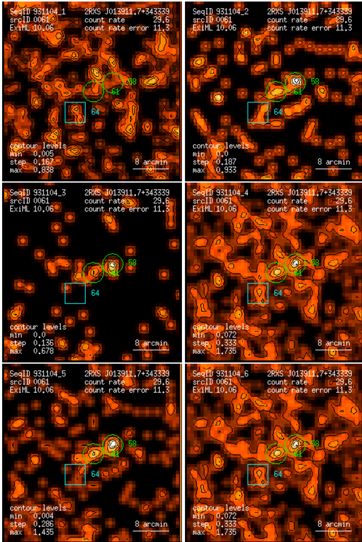
Figure 61: RASS 931104: detection 0061: band rate images, Gaussian filter: (1) PSPC channels 11 – 41, (2) 52 – 90, (3) 91 – 201, (4) 11 – 235, (5) 52 – 201, (6) 11 – 201. Broad band rates in counts/ks. Band rate contour levels in counts/ks/arcmin 2 .
