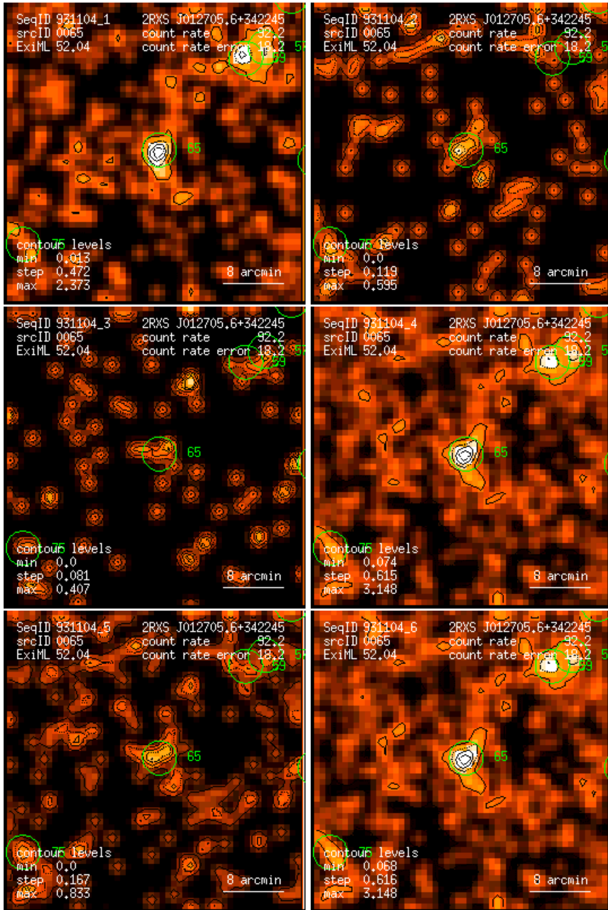
Figure 65: RASS 931104: detection 0065: band rate images, Gaussian filter: (1) PSPC channels 11 – 41, (2) 52 – 90, (3) 91 – 201, (4) 11 – 235, (5) 52 – 201, (6) 11 – 201. Broad band rates in counts/ks. Band rate contour levels in counts/ks/arcmin 2 .
