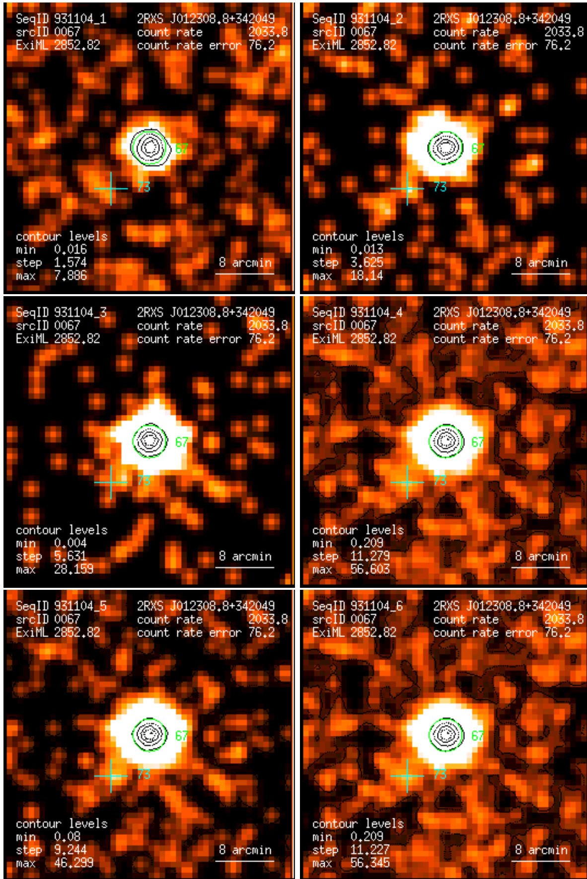
Figure 67: RASS 931104: detection 0067: band rate images, Gaussian filter: (1) PSPC channels 11 – 41, (2) 52 – 90, (3) 91 – 201, (4) 11 – 235, (5) 52 – 201, (6) 11 – 201. Broad band rates in counts/ks. Band rate contour levels in counts/ks/arcmin 2 .
