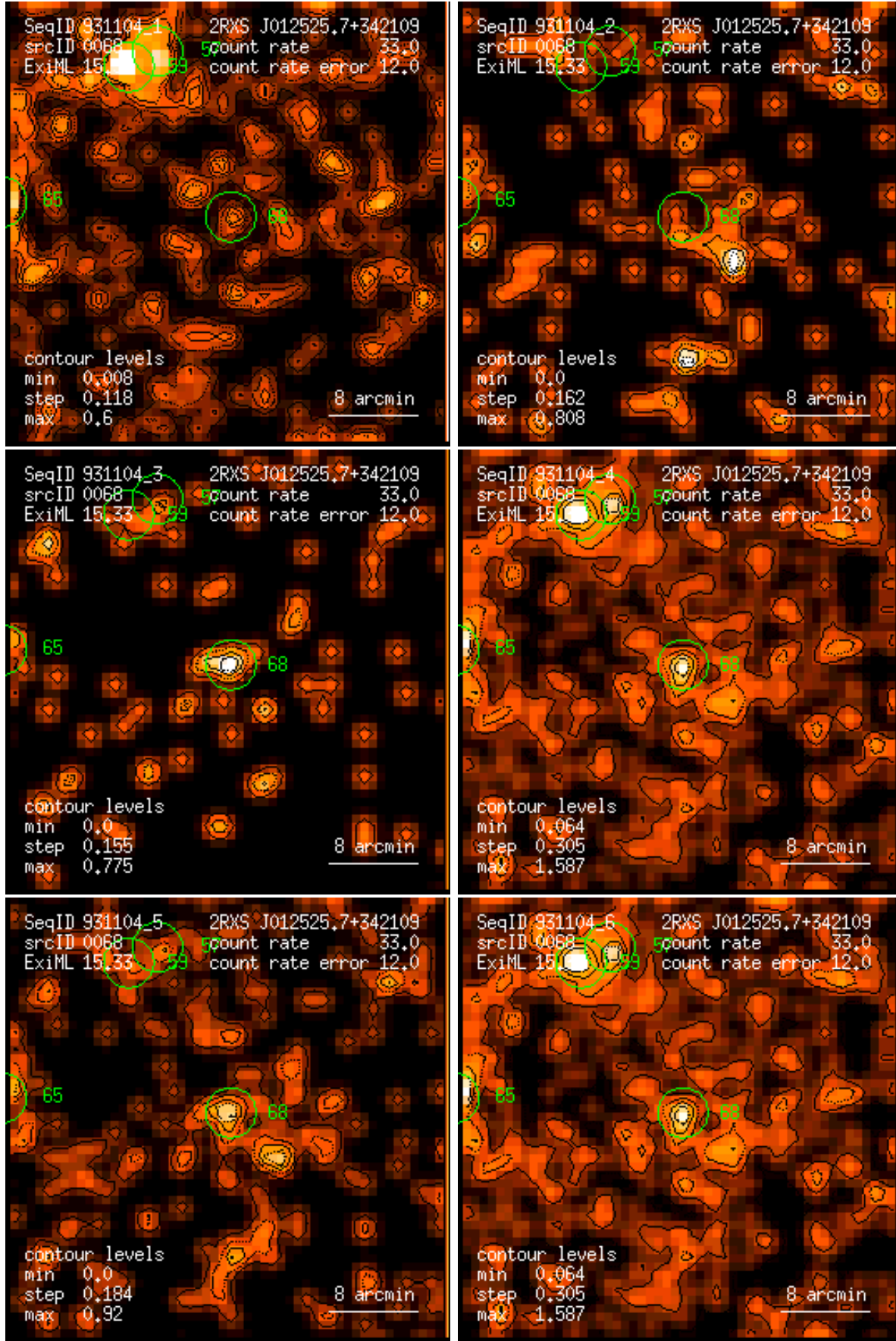
Figure 68: RASS 931104: detection 0068: band rate images, Gaussian filter: (1) PSPC channels 11 – 41, (2) 52 – 90, (3) 91 – 201, (4) 11 – 235, (5) 52 – 201, (6) 11 – 201. Broad band rates in counts/ks. Band rate contour levels in counts/ks/arcmin 2 .
