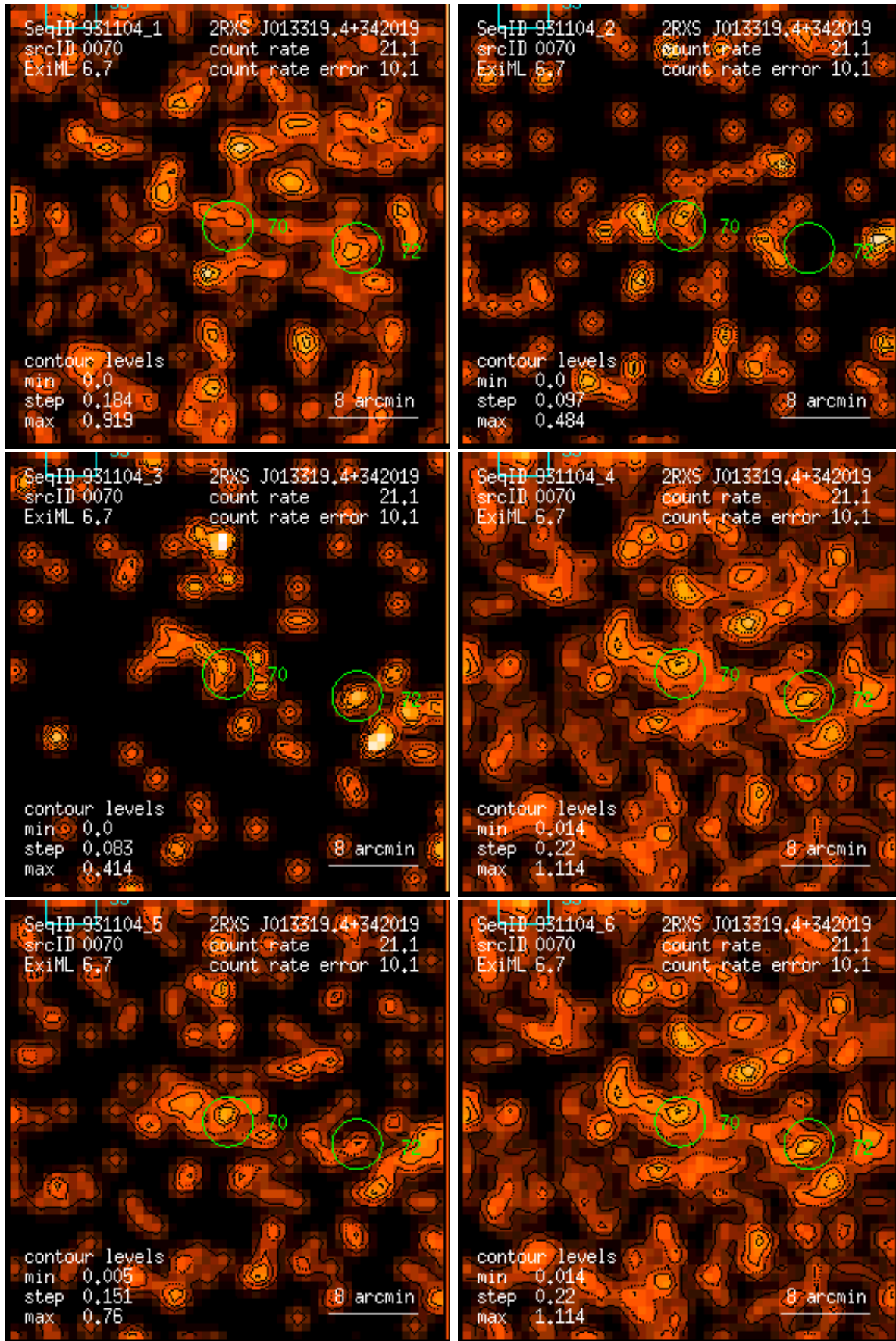
Figure 70: RASS 931104: detection 0070: band rate images, Gaussian filter: (1) PSPC channels 11 – 41, (2) 52 – 90, (3) 91 – 201, (4) 11 – 235, (5) 52 – 201, (6) 11 – 201. Broad band rates in counts/ks. Band rate contour levels in counts/ks/arcmin 2 .
