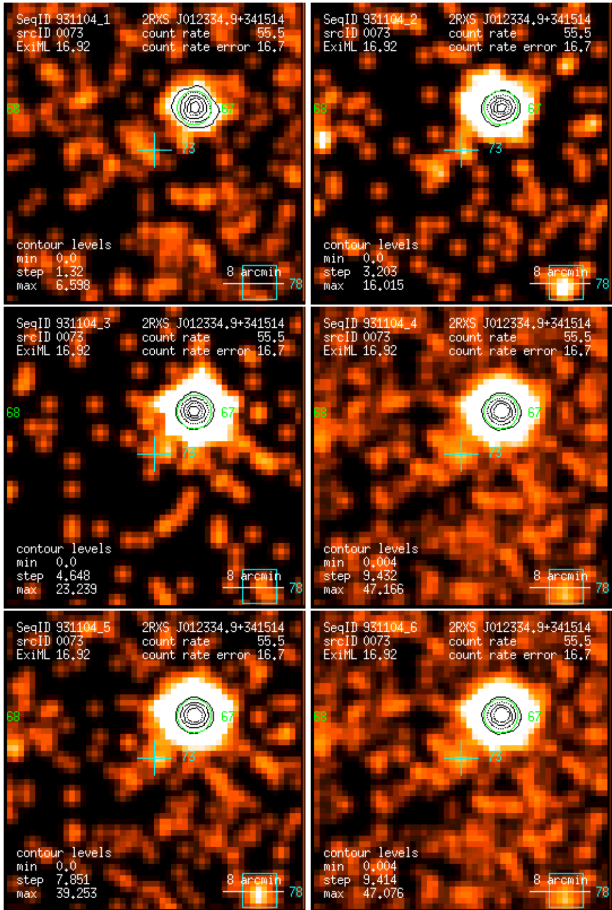
Figure 73: RASS 931104: detection 0073: band rate images, Gaussian filter: (1) PSPC channels 11 – 41, (2) 52 – 90, (3) 91 – 201, (4) 11 – 235, (5) 52 – 201, (6) 11 – 201. Broad band rates in counts/ks. Band rate contour levels in counts/ks/arcmin 2 .
