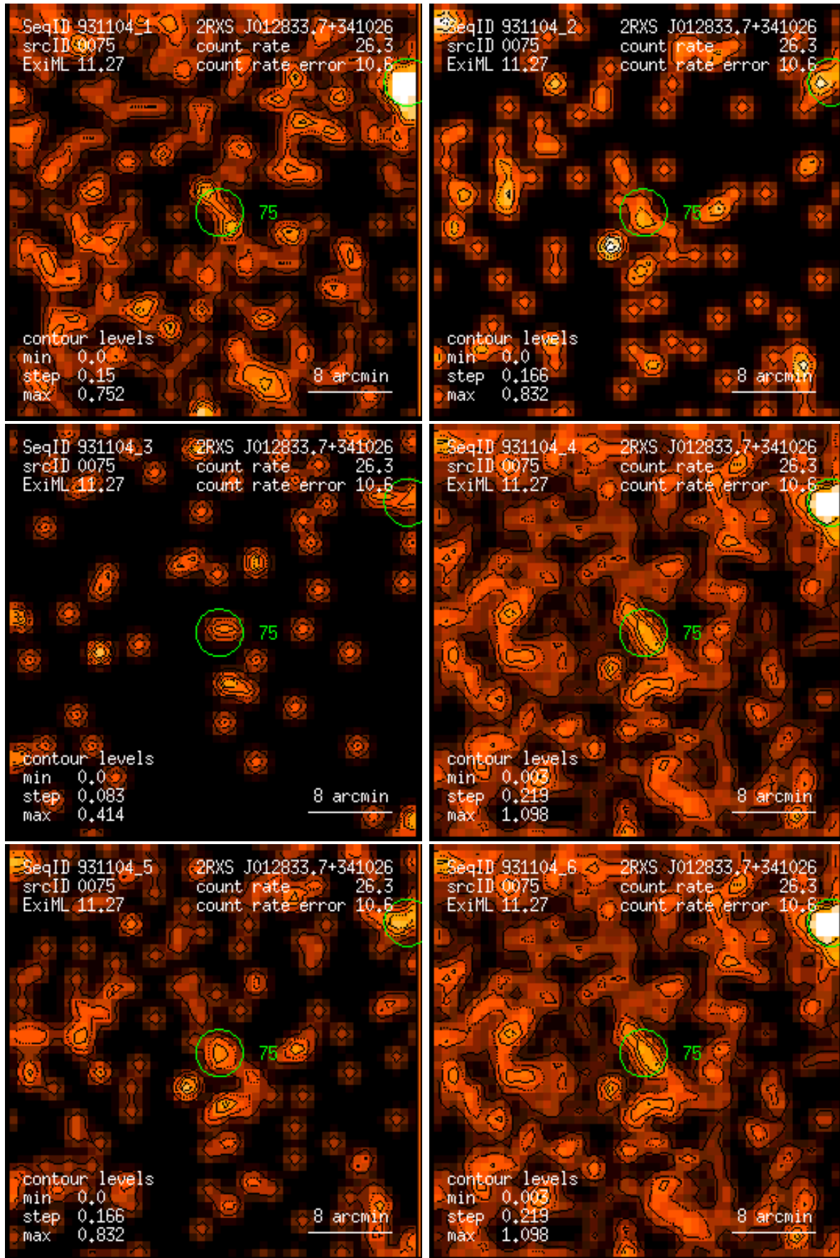
Figure 75: RASS 931104: detection 0075: band rate images, Gaussian filter: (1) PSPC channels 11 – 41, (2) 52 – 90, (3) 91 – 201, (4) 11 – 235, (5) 52 – 201, (6) 11 – 201. Broad band rates in counts/ks. Band rate contour levels in counts/ks/arcmin 2 .
