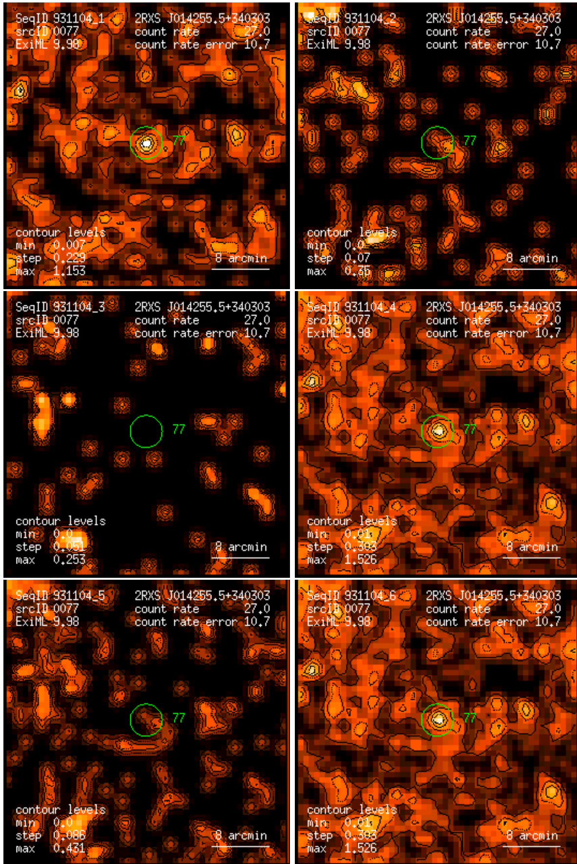
Figure 77: RASS 931104: detection 0077: band rate images, Gaussian filter: (1) PSPC channels 11 – 41, (2) 52 – 90, (3) 91 – 201, (4) 11 – 235, (5) 52 – 201, (6) 11 – 201. Broad band rates in counts/ks. Band rate contour levels in counts/ks/arcmin 2 .
