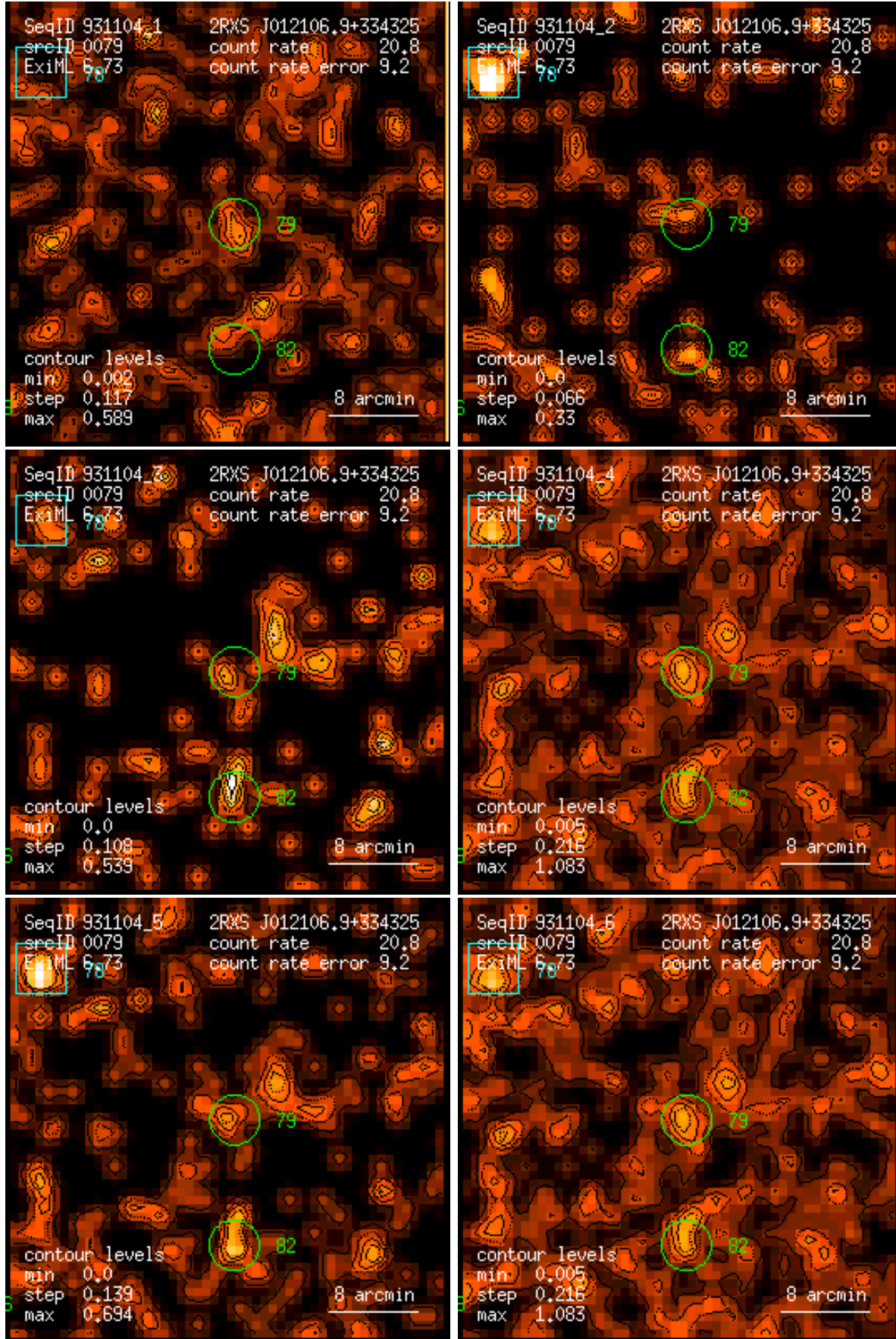
Figure 79: RASS 931104: detection 0079: band rate images, Gaussian filter: (1) PSPC channels 11 – 41, (2) 52 – 90, (3) 91 – 201, (4) 11 – 235, (5) 52 – 201, (6) 11 – 201. Broad band rates in counts/ks. Band rate contour levels in counts/ks/arcmin 2 .
