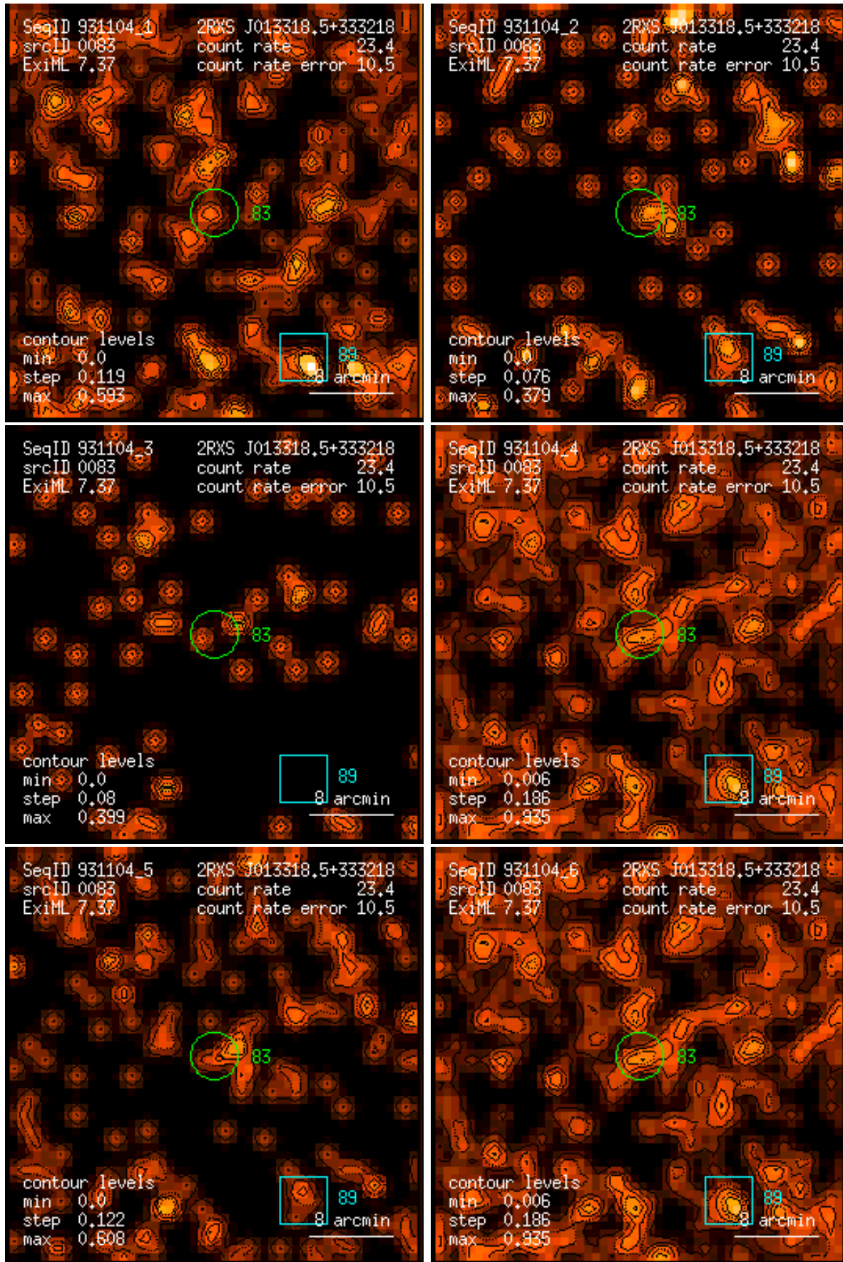
Figure 83: RASS 931104: detection 0083: band rate images, Gaussian filter: (1) PSPC channels 11 – 41, (2) 52 – 90, (3) 91 – 201, (4) 11 – 235, (5) 52 – 201, (6) 11 – 201. Broad band rates in counts/ks. Band rate contour levels in counts/ks/arcmin 2 .
