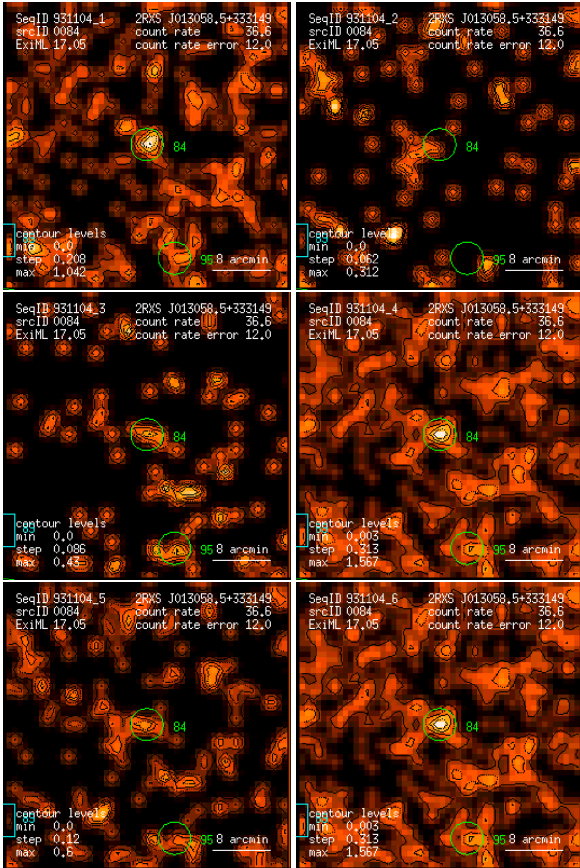
Figure 84: RASS 931104: detection 0084: band rate images, Gaussian filter: (1) PSPC channels 11 – 41, (2) 52 – 90, (3) 91 – 201, (4) 11 – 235, (5) 52 – 201, (6) 11 – 201. Broad band rates in counts/ks. Band rate contour levels in counts/ks/arcmin 2 .
