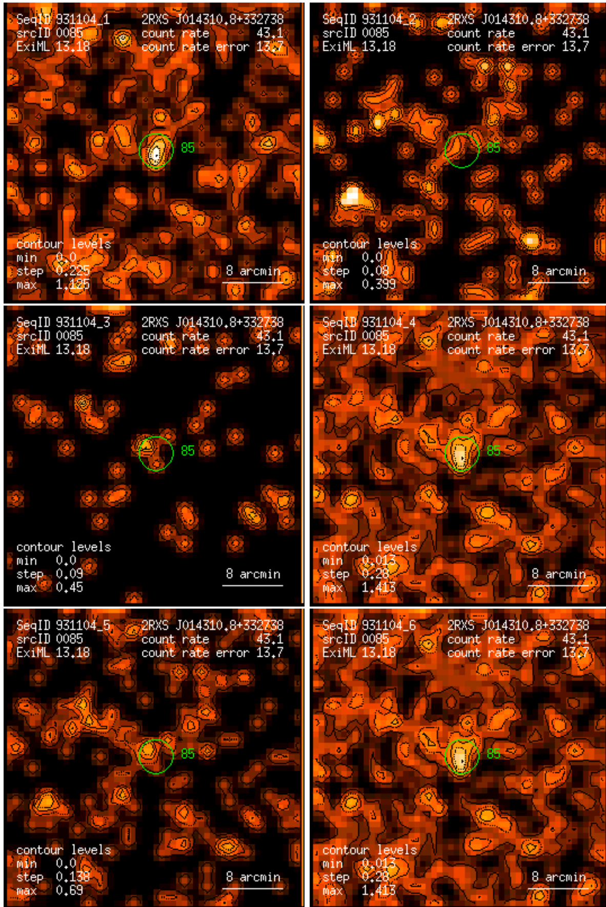
Figure 85: RASS 931104: detection 0085: band rate images, Gaussian filter: (1) PSPC channels 11 – 41, (2) 52 – 90, (3) 91 – 201, (4) 11 – 235, (5) 52 – 201, (6) 11 – 201. Broad band rates in counts/ks. Band rate contour levels in counts/ks/arcmin 2 .
