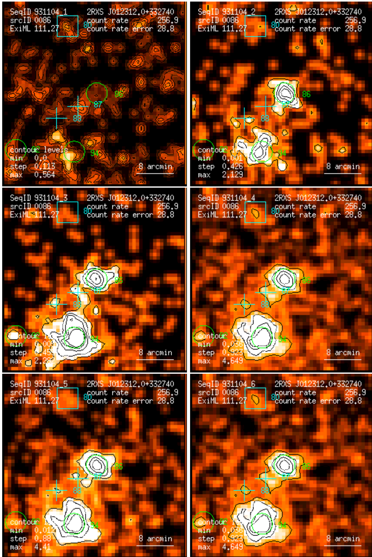
Figure 86: RASS 931104: detection 0086: band rate images, Gaussian filter: (1) PSPC channels 11 – 41, (2) 52 – 90, (3) 91 – 201, (4) 11 – 235, (5) 52 – 201, (6) 11 – 201. Broad band rates in counts/ks. Band rate contour levels in counts/ks/arcmin 2 .
