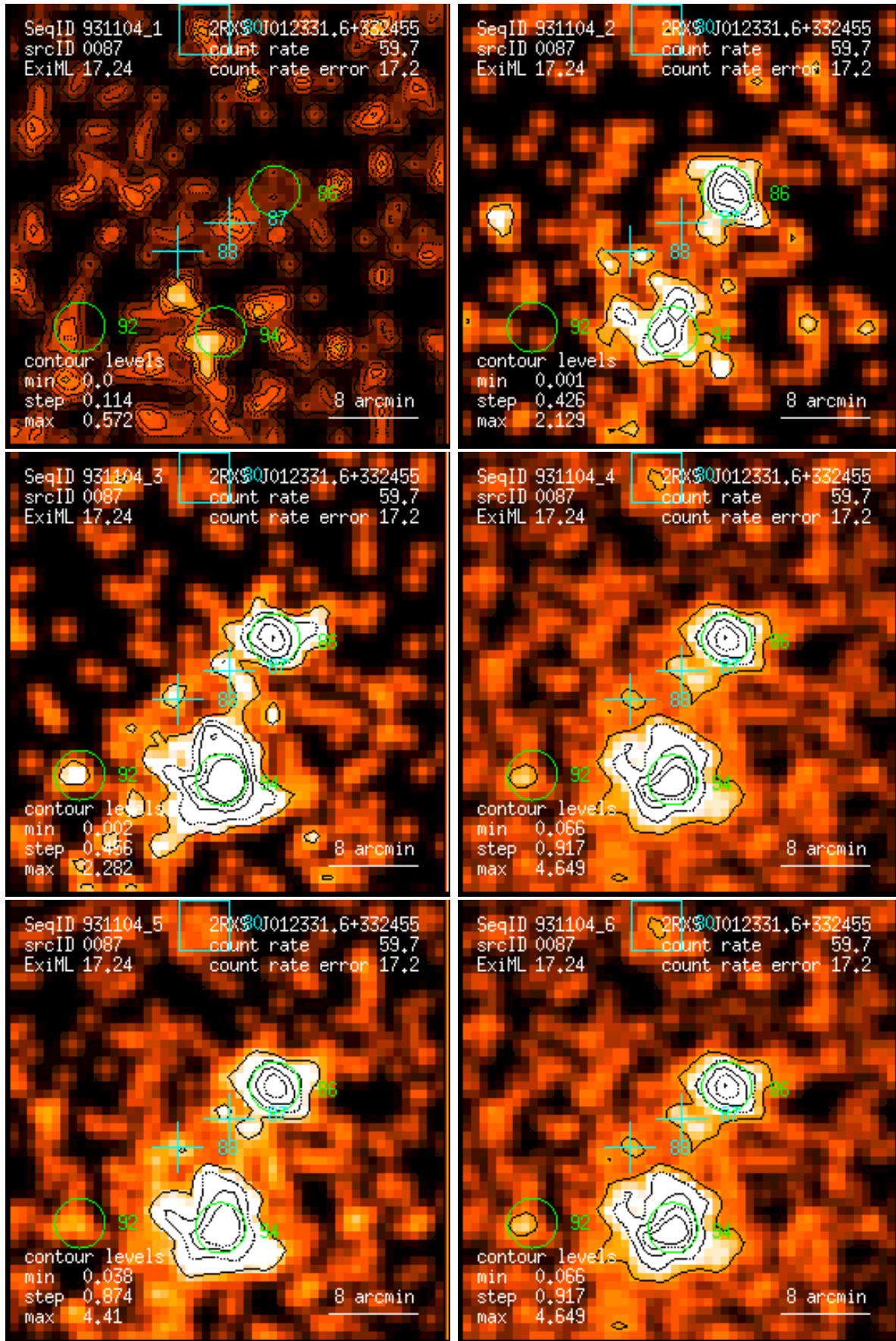
Figure 87: RASS 931104: detection 0087: band rate images, Gaussian filter: (1) PSPC channels 11 – 41, (2) 52 – 90, (3) 91 – 201, (4) 11 – 235, (5) 52 – 201, (6) 11 – 201. Broad band rates in counts/ks. Band rate contour levels in counts/ks/arcmin 2 .
