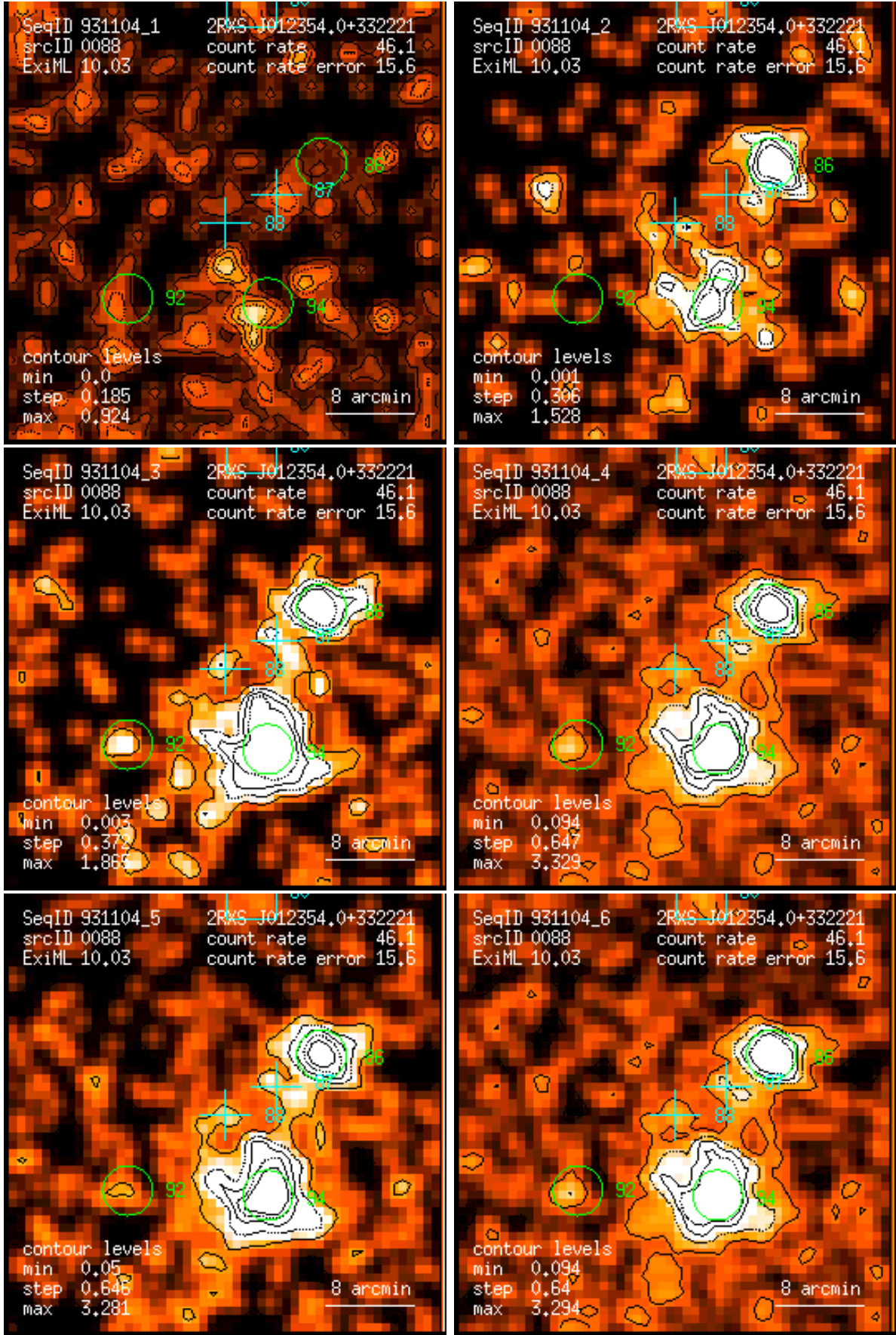
Figure 88: RASS 931104: detection 0088: band rate images, Gaussian filter: (1) PSPC channels 11 – 41, (2) 52 – 90, (3) 91 – 201, (4) 11 – 235, (5) 52 – 201, (6) 11 – 201. Broad band rates in counts/ks. Band rate contour levels in counts/ks/arcmin 2 .
