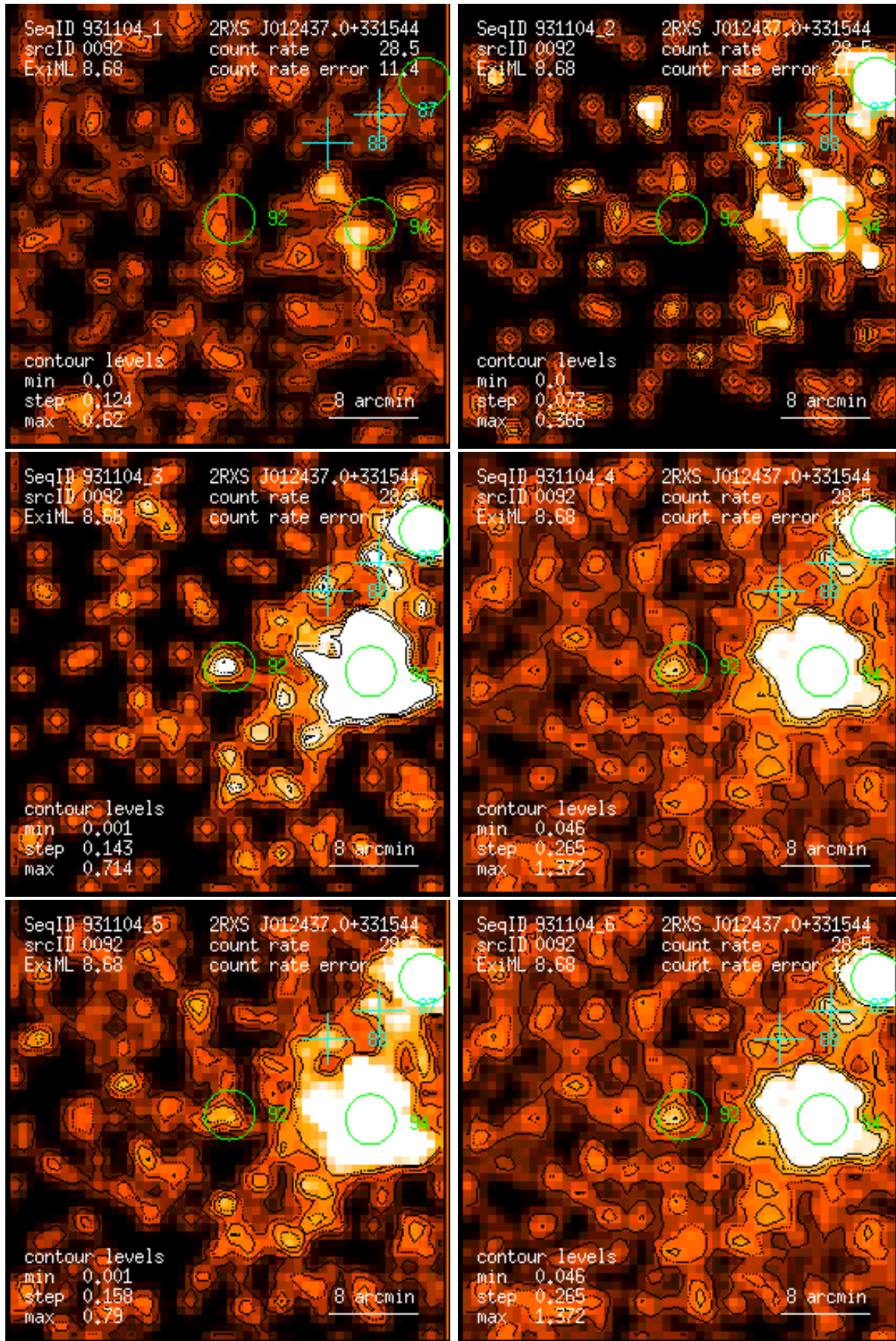
Figure 92: RASS 931104: detection 0092: band rate images, Gaussian filter: (1) PSPC channels 11 – 41, (2) 52 – 90, (3) 91 – 201, (4) 11 – 235, (5) 52 – 201, (6) 11 – 201. Broad band rates in counts/ks. Band rate contour levels in counts/ks/arcmin 2 .
