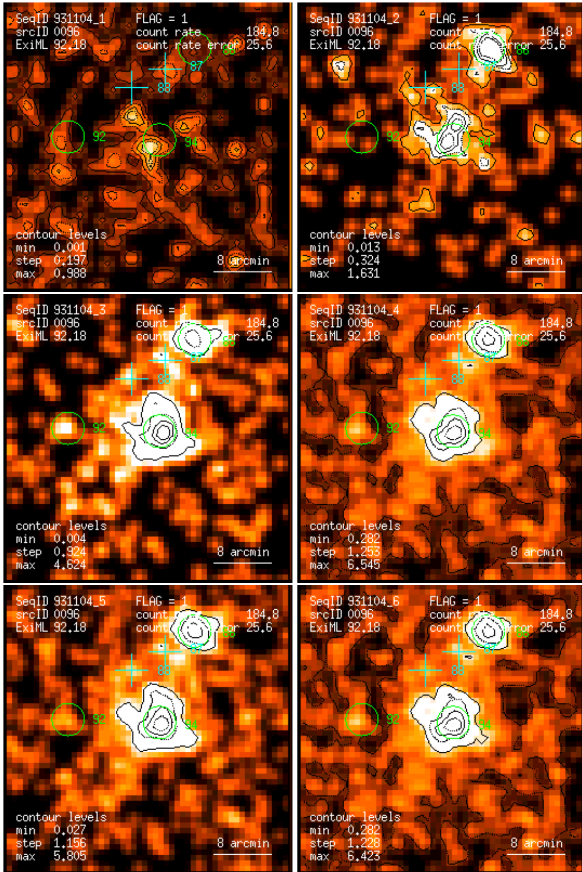
Figure 96: RASS 931104: detection 0096: band rate images, Gaussian filter: (1) PSPC channels 11 – 41, (2) 52 – 90, (3) 91 – 201, (4) 11 – 235, (5) 52 – 201, (6) 11 – 201. Broad band rates in counts/ks. Band rate contour levels in counts/ks/arcmin 2 .
