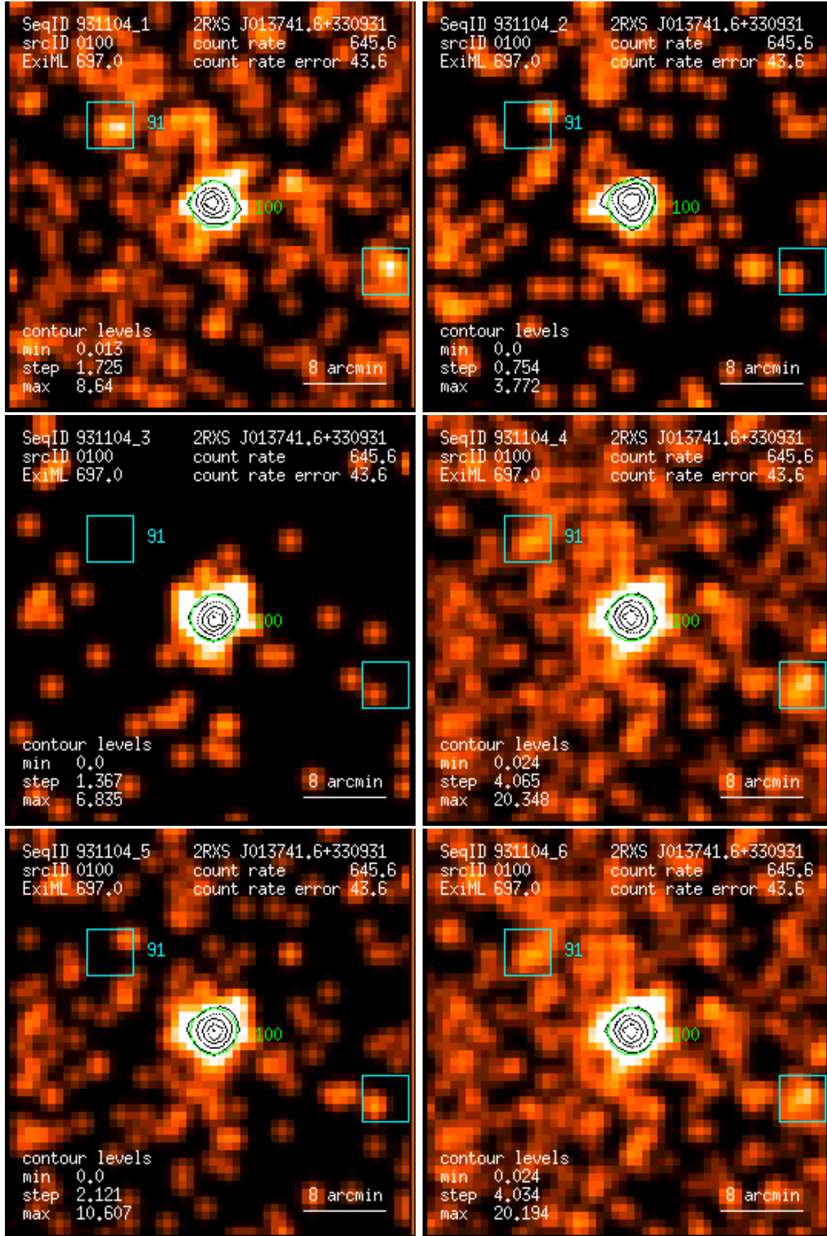
Figure 100: RASS 931104: detection 0100: band rate images, Gaussian filter: (1) PSPC channels 11 – 41, (2) 52 – 90, (3) 91 – 201, (4) 11 – 235, (5) 52 – 201, (6) 11 – 201. Broad band rates in counts/ks. Band rate contour levels in counts/ks/arcmin 2 .
