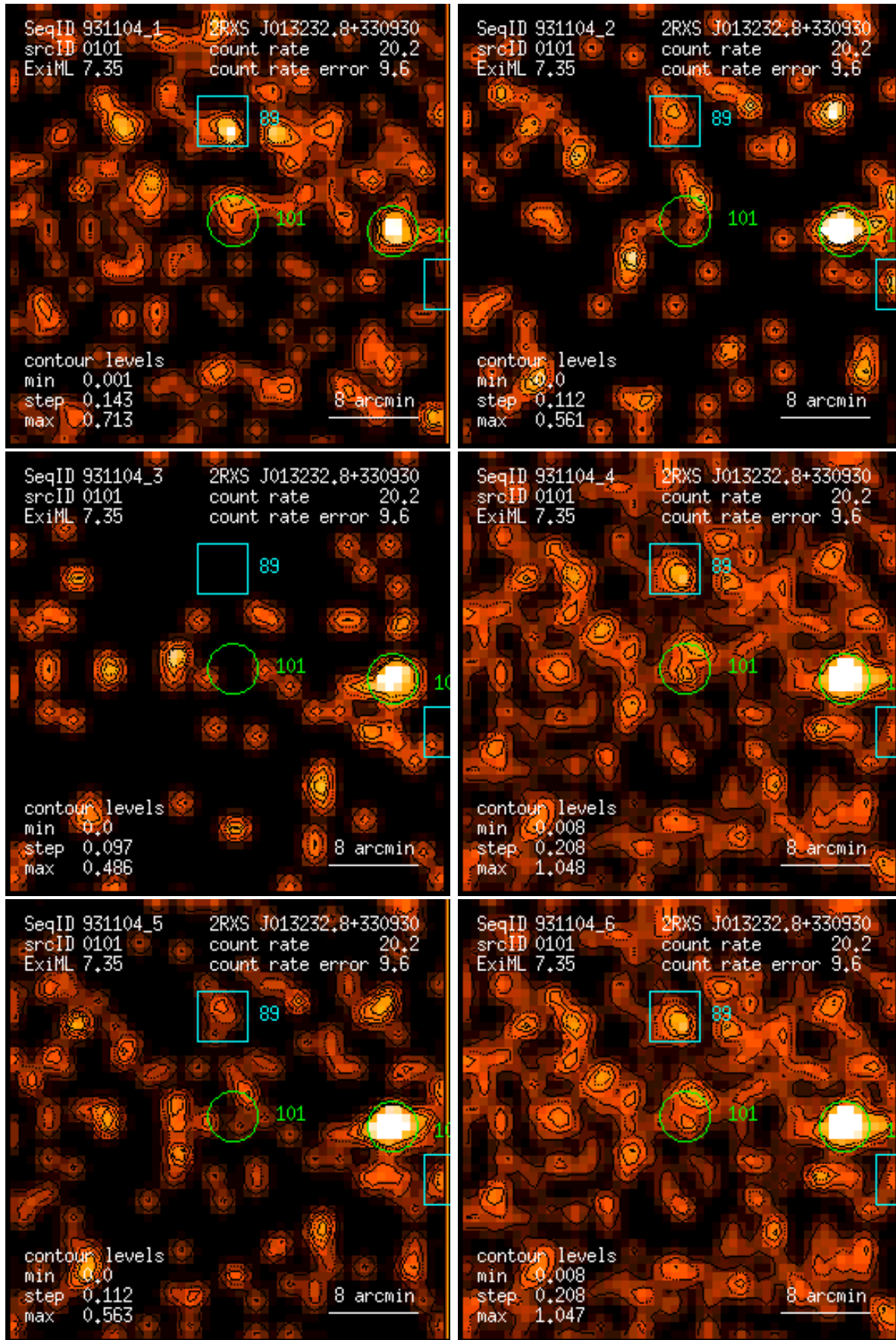
Figure 101: RASS 931104: detection 0101: band rate images, Gaussian filter: (1) PSPC channels 11 – 41, (2) 52 – 90, (3) 91 – 201, (4) 11 – 235, (5) 52 – 201, (6) 11 – 201. Broad band rates in counts/ks. Band rate contour levels in counts/ks/arcmin 2 .
