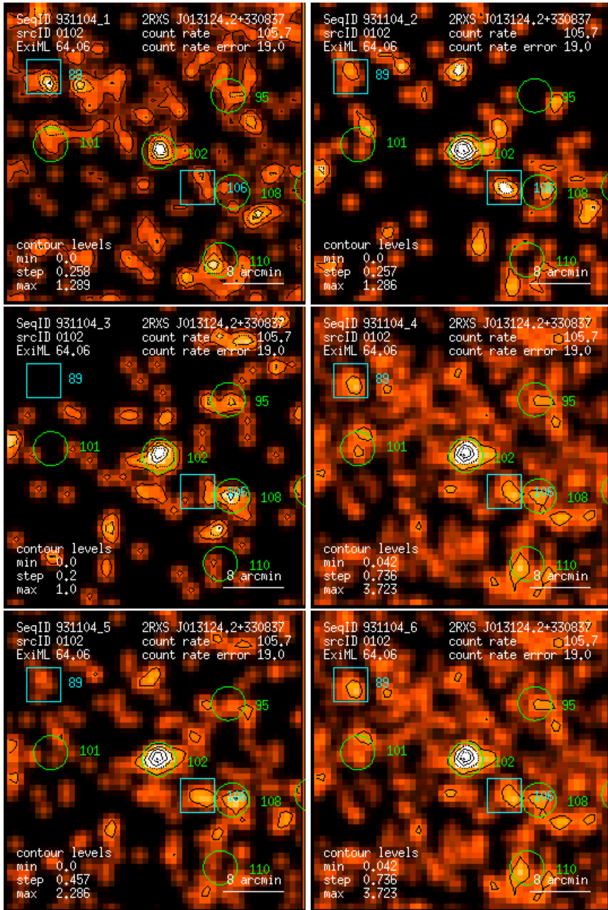
Figure 102: RASS 931104: detection 0102: band rate images, Gaussian filter: (1) PSPC channels 11 – 41, (2) 52 – 90, (3) 91 – 201, (4) 11 – 235, (5) 52 – 201, (6) 11 – 201. Broad band rates in counts/ks. Band rate contour levels in counts/ks/arcmin 2 .
