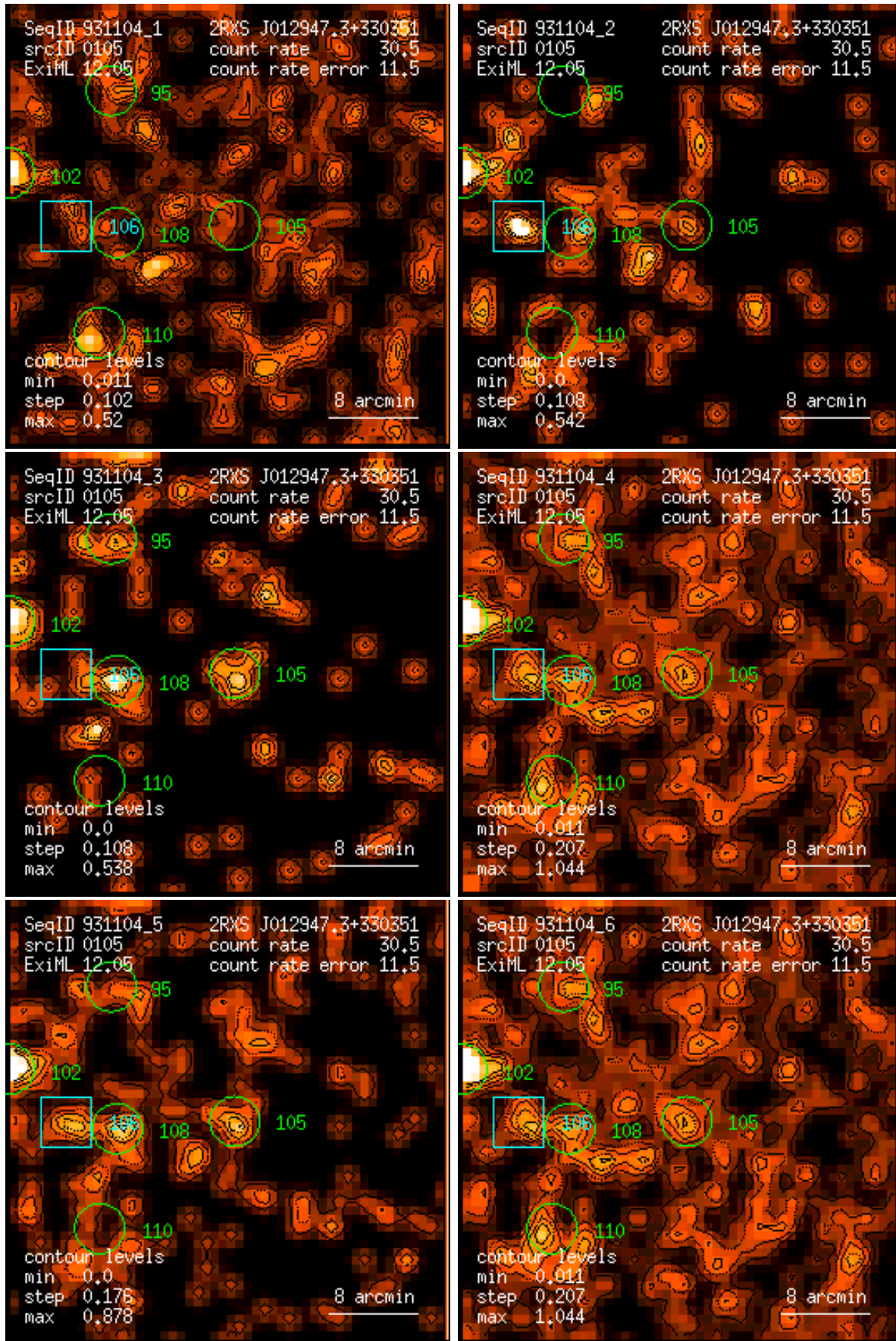
Figure 105: RASS 931104: detection 0105: band rate images, Gaussian filter: (1) PSPC channels 11 – 41, (2) 52 – 90, (3) 91 – 201, (4) 11 – 235, (5) 52 – 201, (6) 11 – 201. Broad band rates in counts/ks. Band rate contour levels in counts/ks/arcmin 2 .
