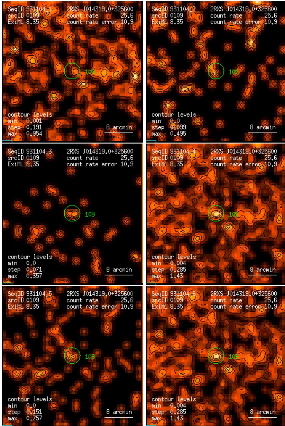
Figure 109: RASS 931104: detection 0109: band rate images, Gaussian filter: (1) PSPC channels 11 – 41, (2) 52 – 90, (3) 91 – 201, (4) 11 – 235, (5) 52 – 201, (6) 11 – 201. Broad band rates in counts/ks. Band rate contour levels in counts/ks/arcmin 2 .
