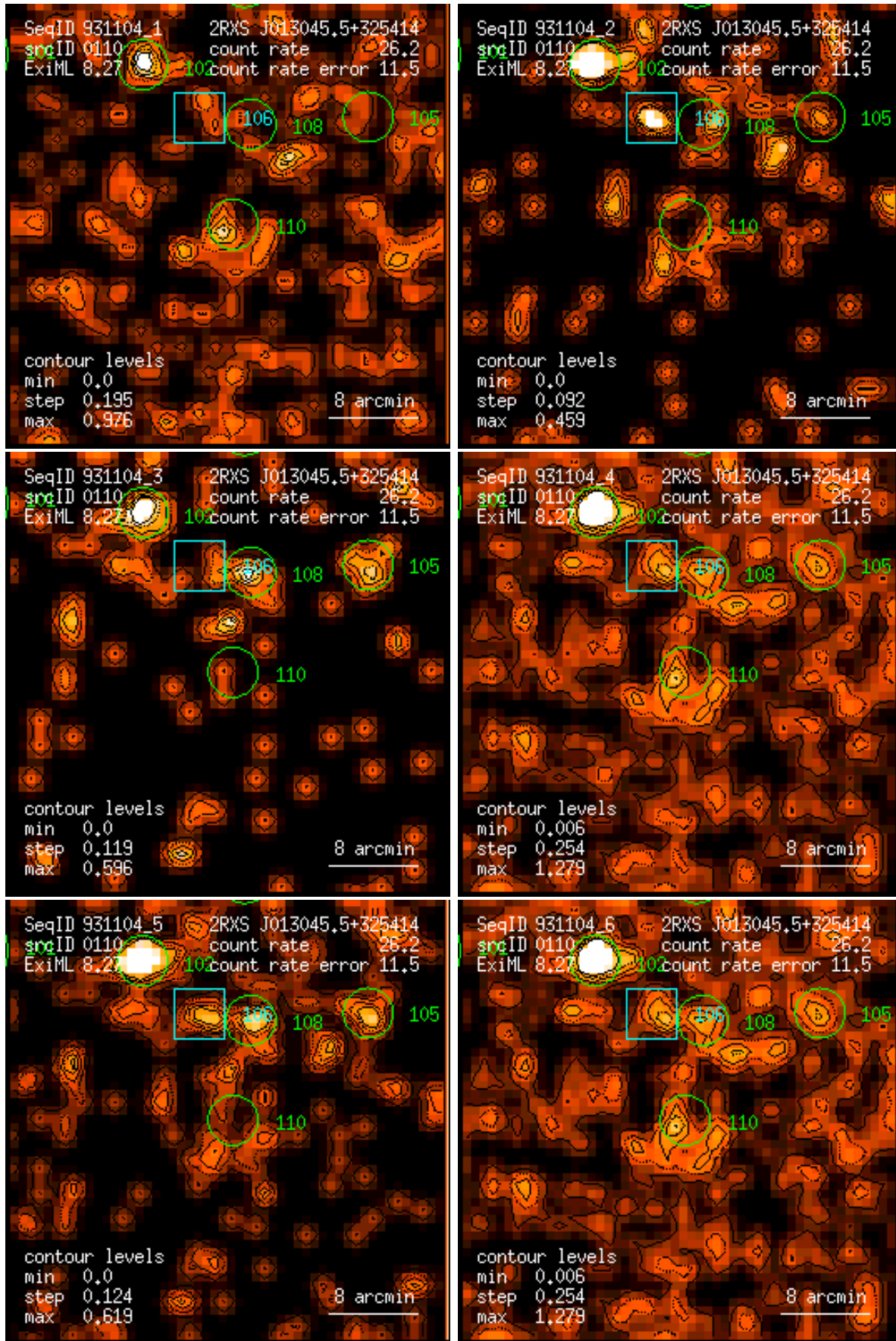
Figure 110: RASS 931104: detection 0110: band rate images, Gaussian filter: (1) PSPC channels 11 – 41, (2) 52 – 90, (3) 91 – 201, (4) 11 – 235, (5) 52 – 201, (6) 11 – 201. Broad band rates in counts/ks. Band rate contour levels in counts/ks/arcmin 2 .
