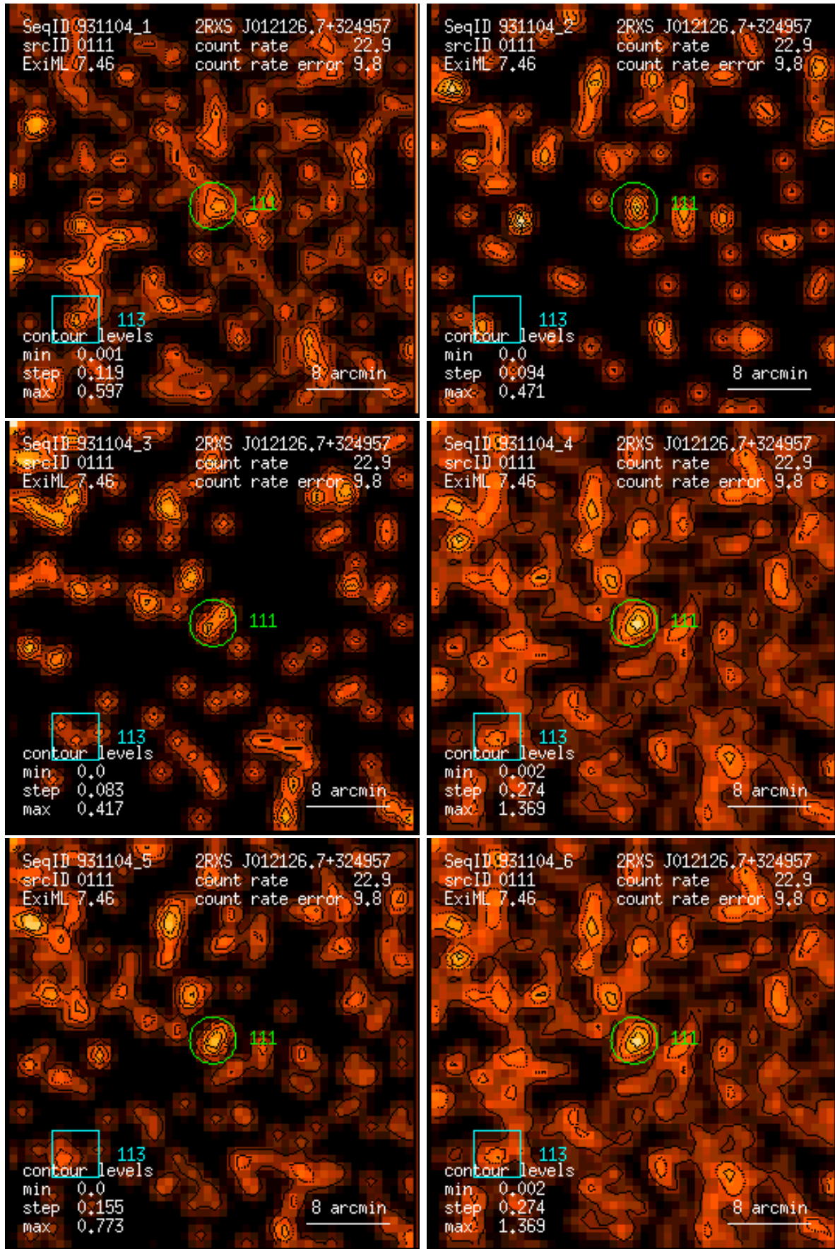
Figure 111: RASS 931104: detection 0111: band rate images, Gaussian filter: (1) PSPC channels 11 – 41, (2) 52 – 90, (3) 91 – 201, (4) 11 – 235, (5) 52 – 201, (6) 11 – 201. Broad band rates in counts/ks. Band rate contour levels in counts/ks/arcmin 2 .
