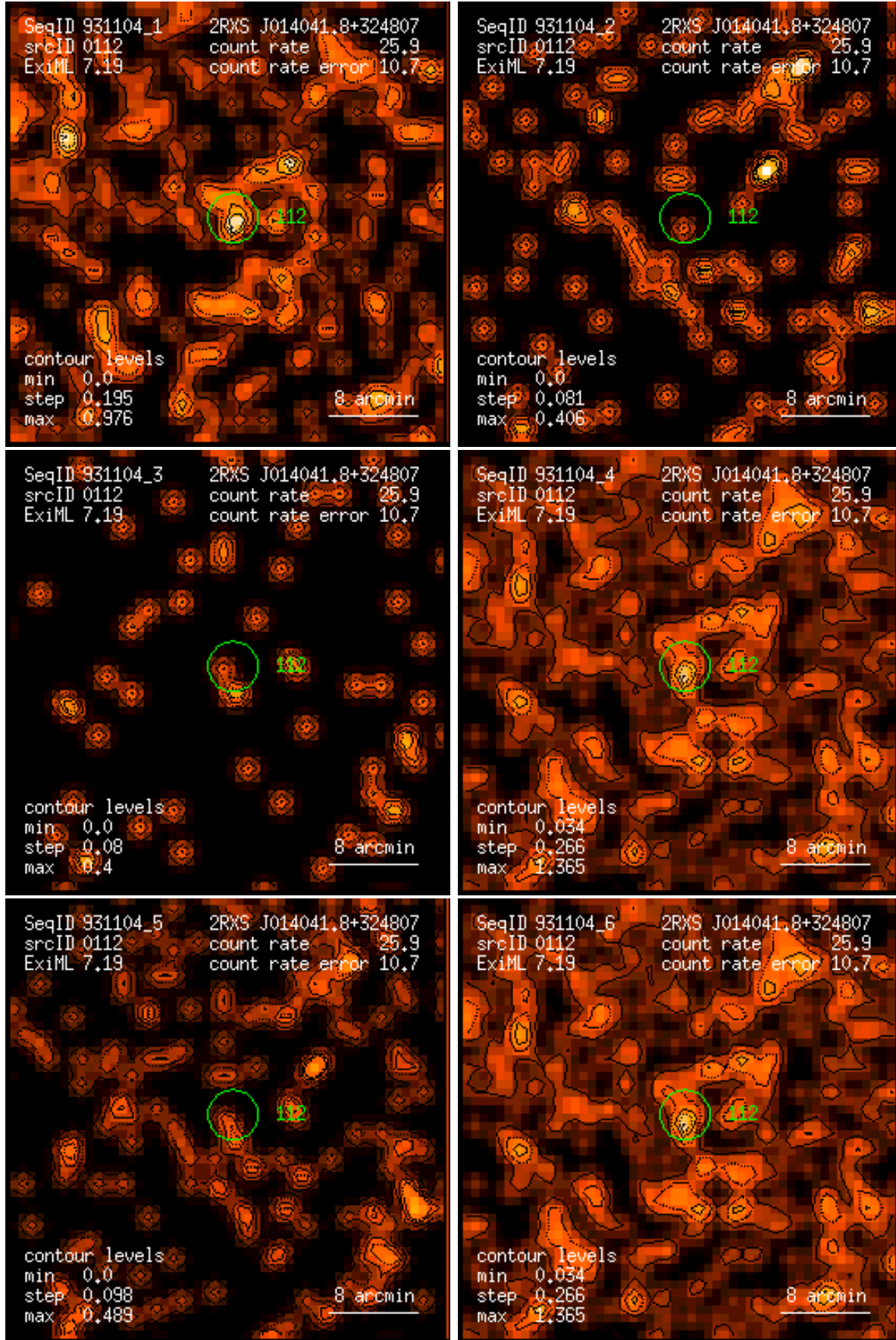
Figure 112: RASS 931104: detection 0112: band rate images, Gaussian filter: (1) PSPC channels 11 – 41, (2) 52 – 90, (3) 91 – 201, (4) 11 – 235, (5) 52 – 201, (6) 11 – 201. Broad band rates in counts/ks. Band rate contour levels in counts/ks/arcmin 2 .
