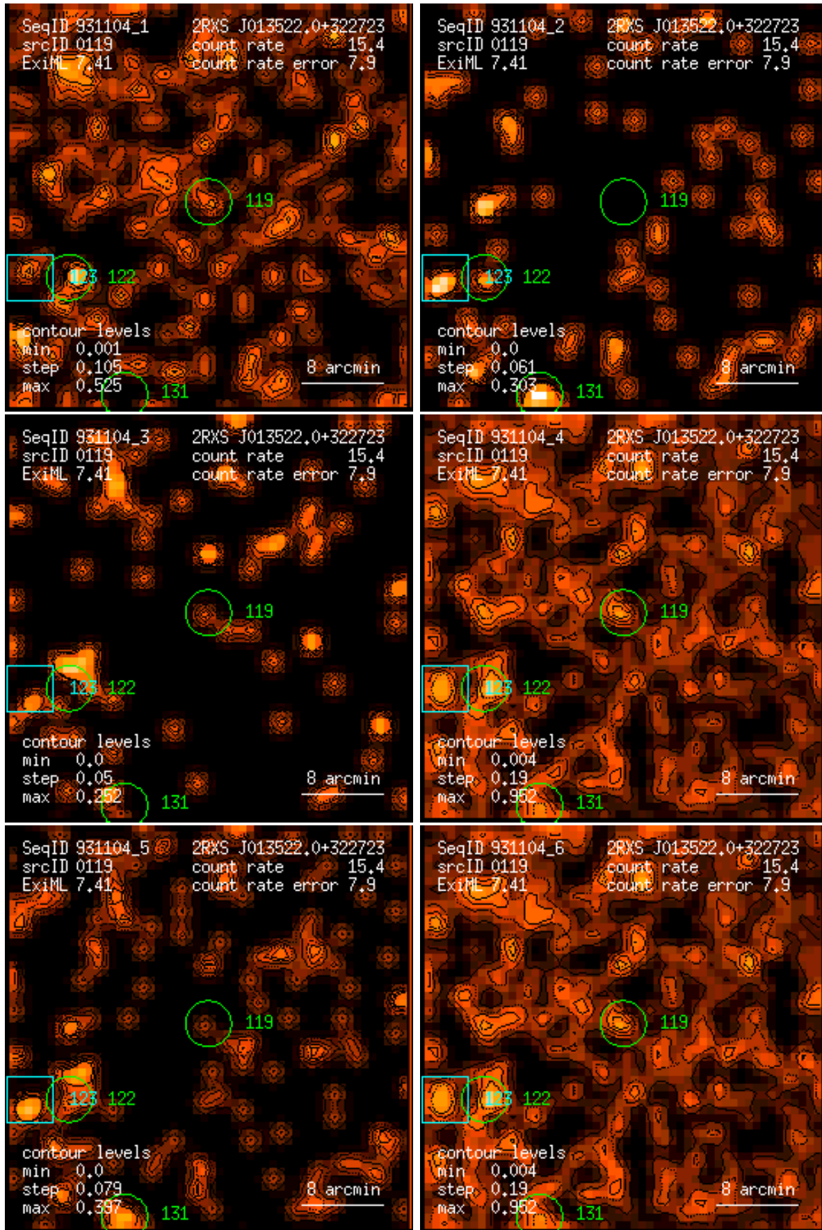
Figure 119: RASS 931104: detection 0119: band rate images, Gaussian filter: (1) PSPC channels 11 – 41, (2) 52 – 90, (3) 91 – 201, (4) 11 – 235, (5) 52 – 201, (6) 11 – 201. Broad band rates in counts/ks. Band rate contour levels in counts/ks/arcmin 2 .
