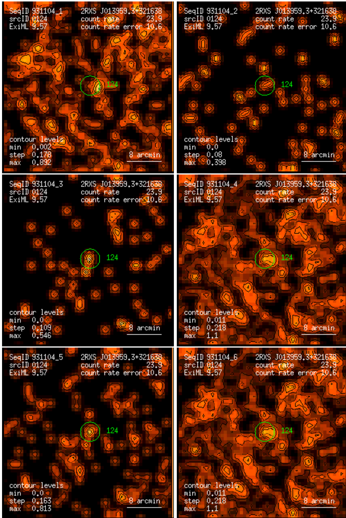
Figure 124: RASS 931104: detection 0124: band rate images, Gaussian filter: (1) PSPC channels 11 – 41, (2) 52 – 90, (3) 91 – 201, (4) 11 – 235, (5) 52 – 201, (6) 11 – 201. Broad band rates in counts/ks. Band rate contour levels in counts/ks/arcmin 2 .
