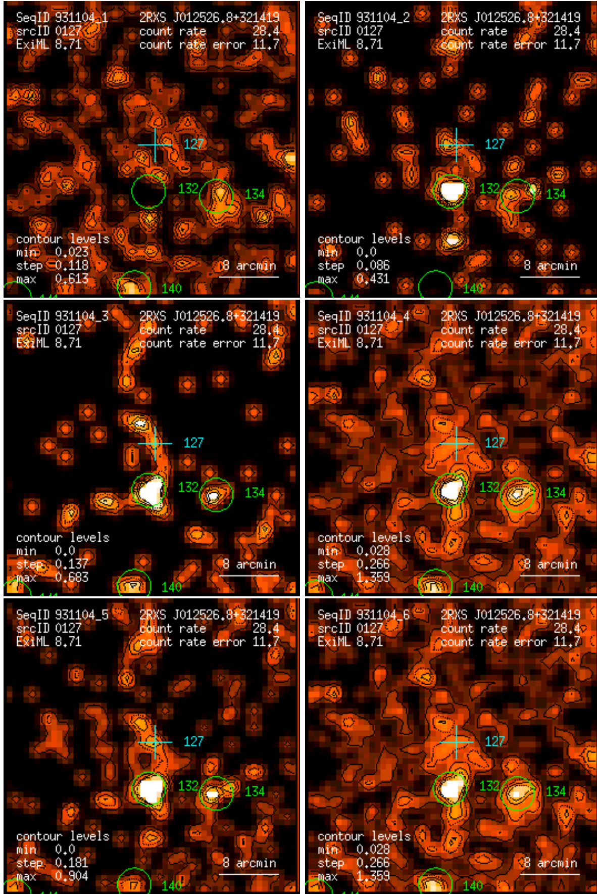
Figure 127: RASS 931104: detection 0127: band rate images, Gaussian filter: (1) PSPC channels 11 – 41, (2) 52 – 90, (3) 91 – 201, (4) 11 – 235, (5) 52 – 201, (6) 11 – 201. Broad band rates in counts/ks. Band rate contour levels in counts/ks/arcmin 2 .
