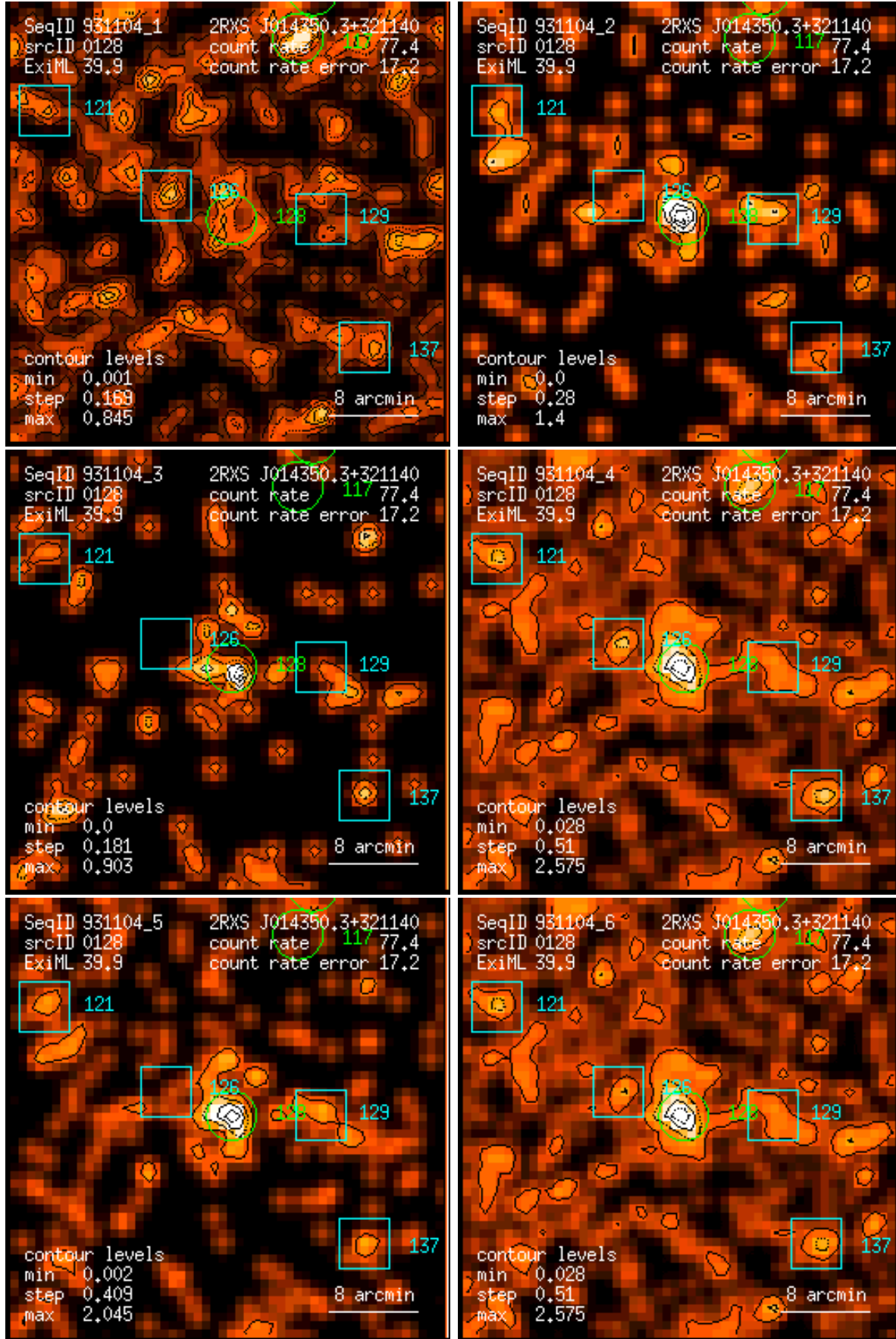
Figure 128: RASS 931104: detection 0128: band rate images, Gaussian filter: (1) PSPC channels 11 – 41, (2) 52 – 90, (3) 91 – 201, (4) 11 – 235, (5) 52 – 201, (6) 11 – 201. Broad band rates in counts/ks. Band rate contour levels in counts/ks/arcmin 2 .
