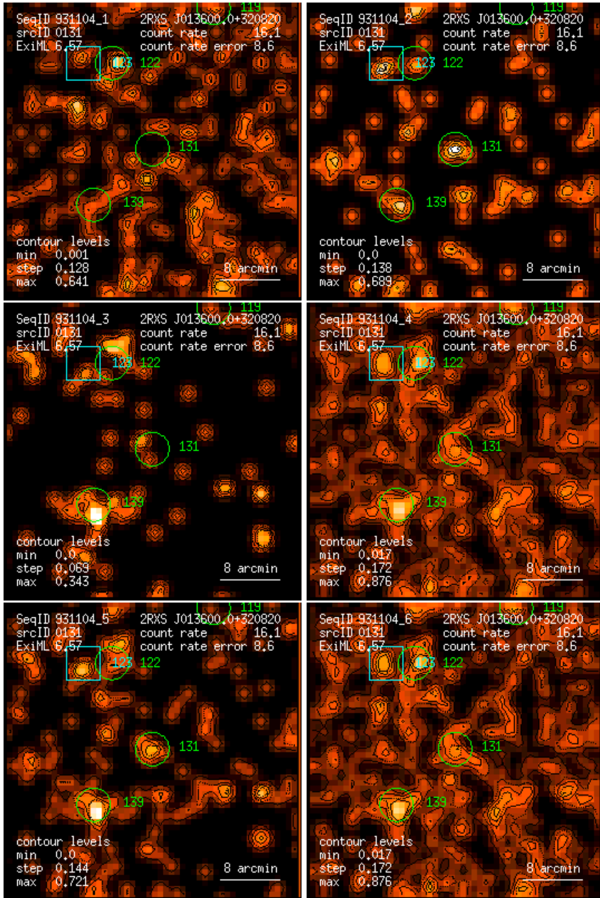
Figure 131: RASS 931104: detection 0131: band rate images, Gaussian filter: (1) PSPC channels 11 – 41, (2) 52 – 90, (3) 91 – 201, (4) 11 – 235, (5) 52 – 201, (6) 11 – 201. Broad band rates in counts/ks. Band rate contour levels in counts/ks/arcmin 2 .
