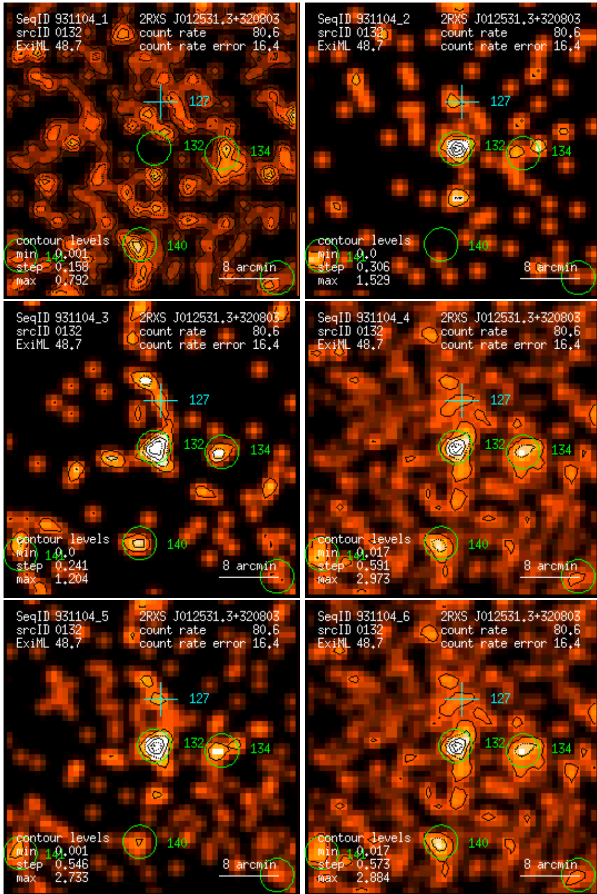
Figure 132: RASS 931104: detection 0132: band rate images, Gaussian filter: (1) PSPC channels 11 – 41, (2) 52 – 90, (3) 91 – 201, (4) 11 – 235, (5) 52 – 201, (6) 11 – 201. Broad band rates in counts/ks. Band rate contour levels in counts/ks/arcmin 2 .
