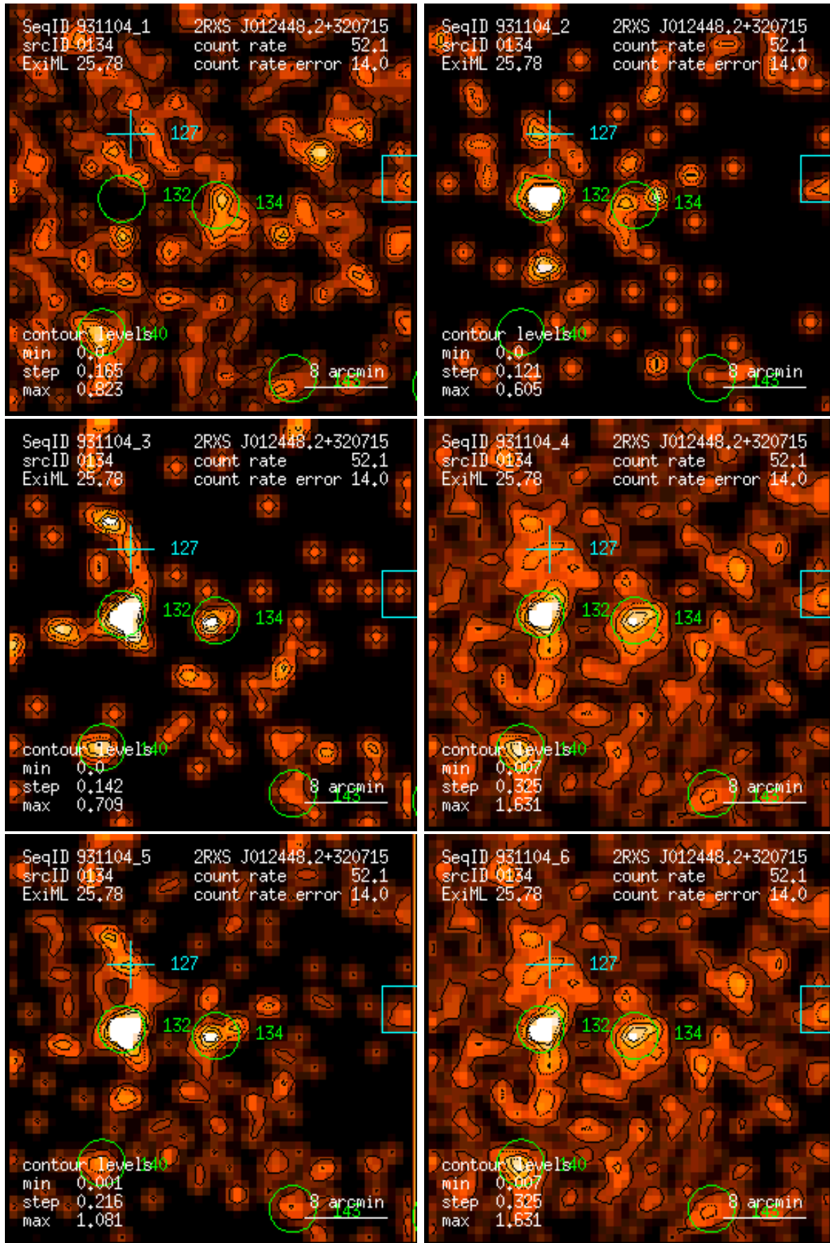
Figure 134: RASS 931104: detection 0134: band rate images, Gaussian filter: (1) PSPC channels 11 – 41, (2) 52 – 90, (3) 91 – 201, (4) 11 – 235, (5) 52 – 201, (6) 11 – 201. Broad band rates in counts/ks. Band rate contour levels in counts/ks/arcmin 2 .
