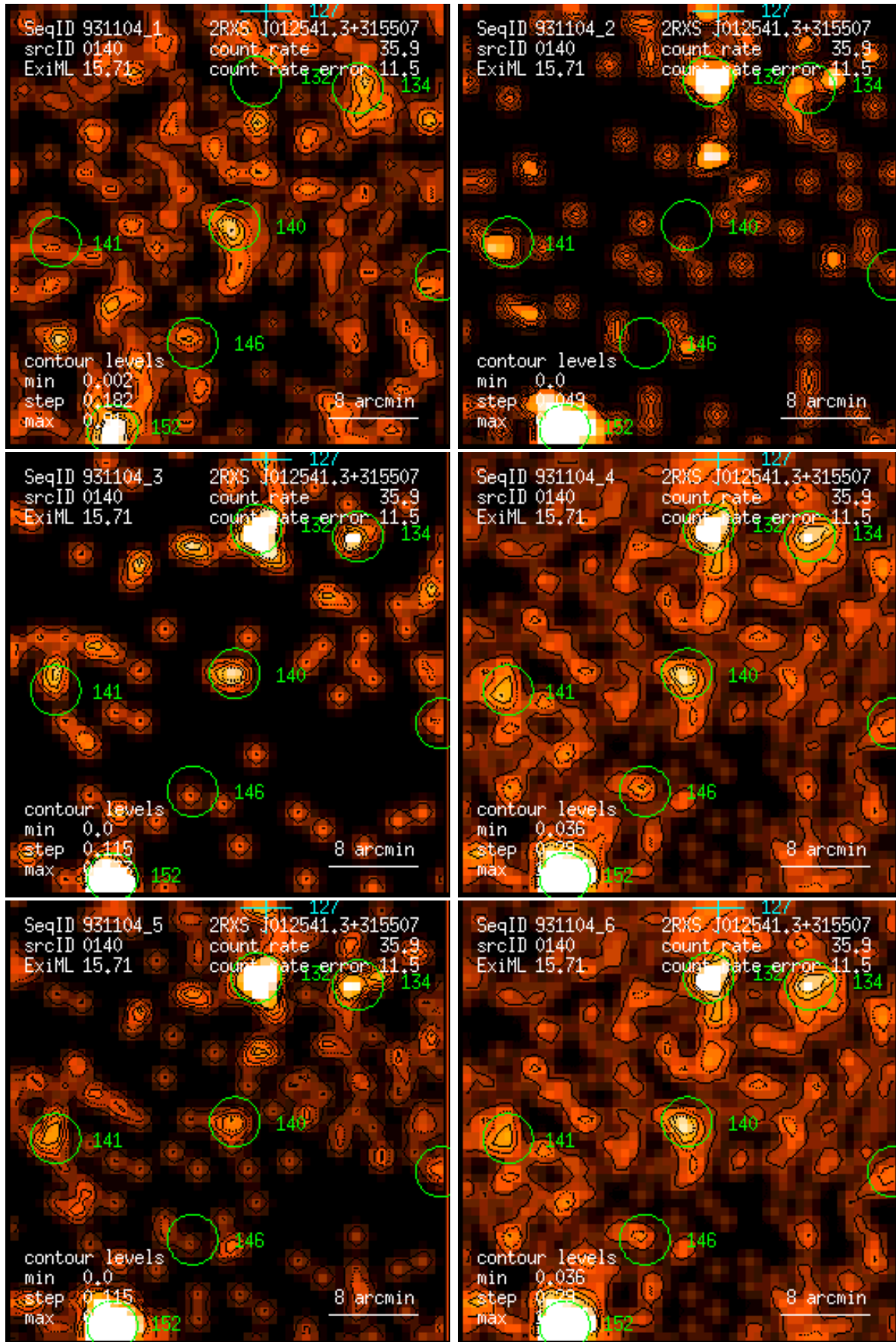
Figure 140: RASS 931104: detection 0140: band rate images, Gaussian filter: (1) PSPC channels 11 – 41, (2) 52 – 90, (3) 91 – 201, (4) 11 – 235, (5) 52 – 201, (6) 11 – 201. Broad band rates in counts/ks. Band rate contour levels in counts/ks/arcmin 2 .
