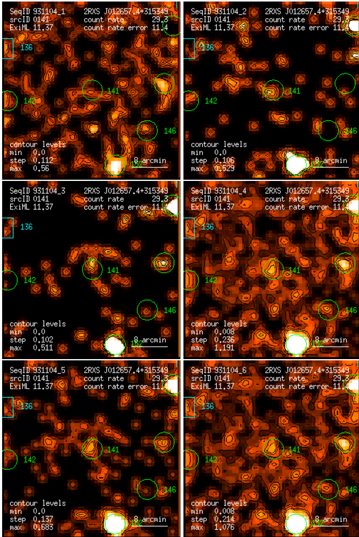
Figure 141: RASS 931104: detection 0141: band rate images, Gaussian filter: (1) PSPC channels 11 – 41, (2) 52 – 90, (3) 91 – 201, (4) 11 – 235, (5) 52 – 201, (6) 11 – 201. Broad band rates in counts/ks. Band rate contour levels in counts/ks/arcmin 2 .
