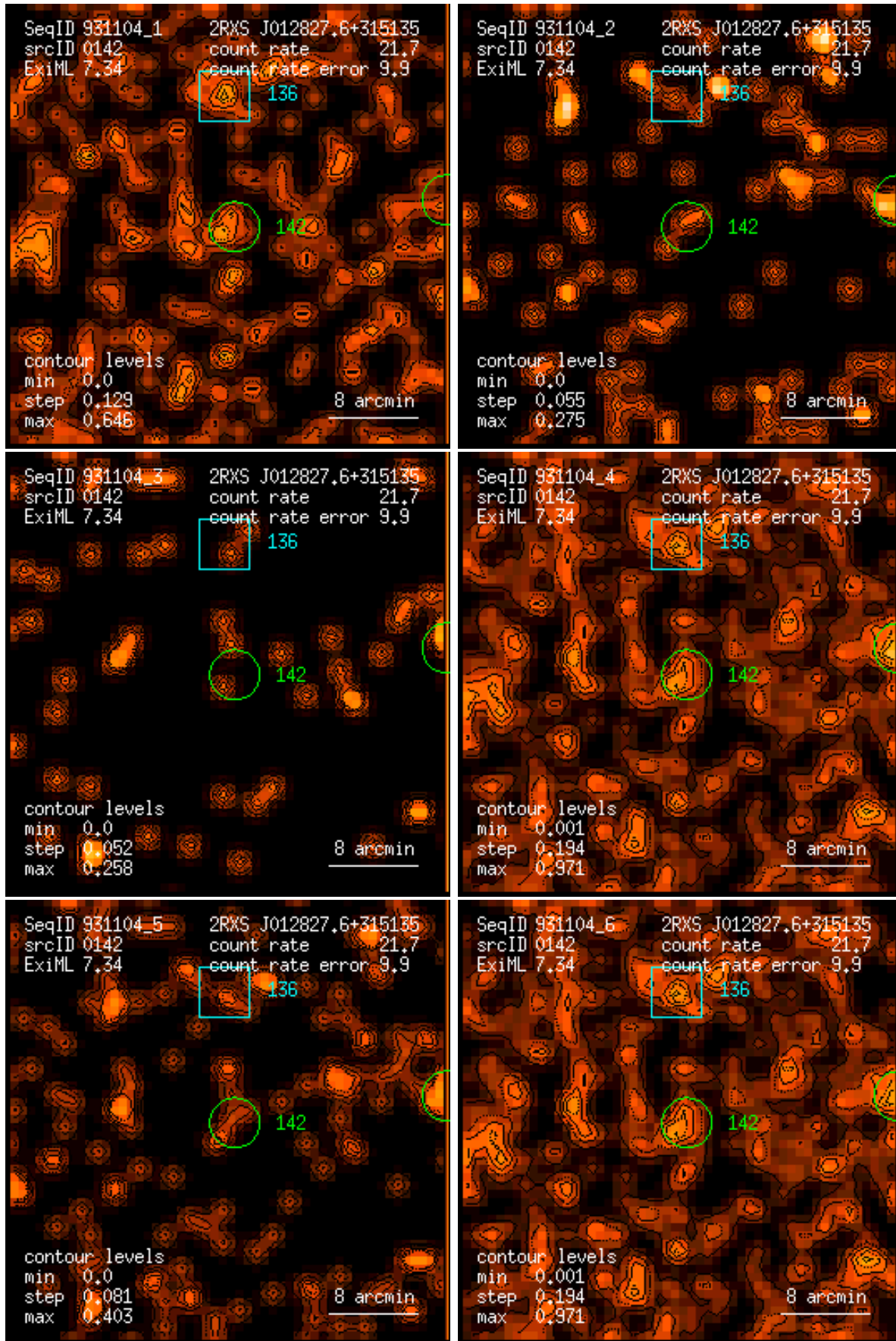
Figure 142: RASS 931104: detection 0142: band rate images, Gaussian filter: (1) PSPC channels 11 – 41, (2) 52 – 90, (3) 91 – 201, (4) 11 – 235, (5) 52 – 201, (6) 11 – 201. Broad band rates in counts/ks. Band rate contour levels in counts/ks/arcmin 2 .
