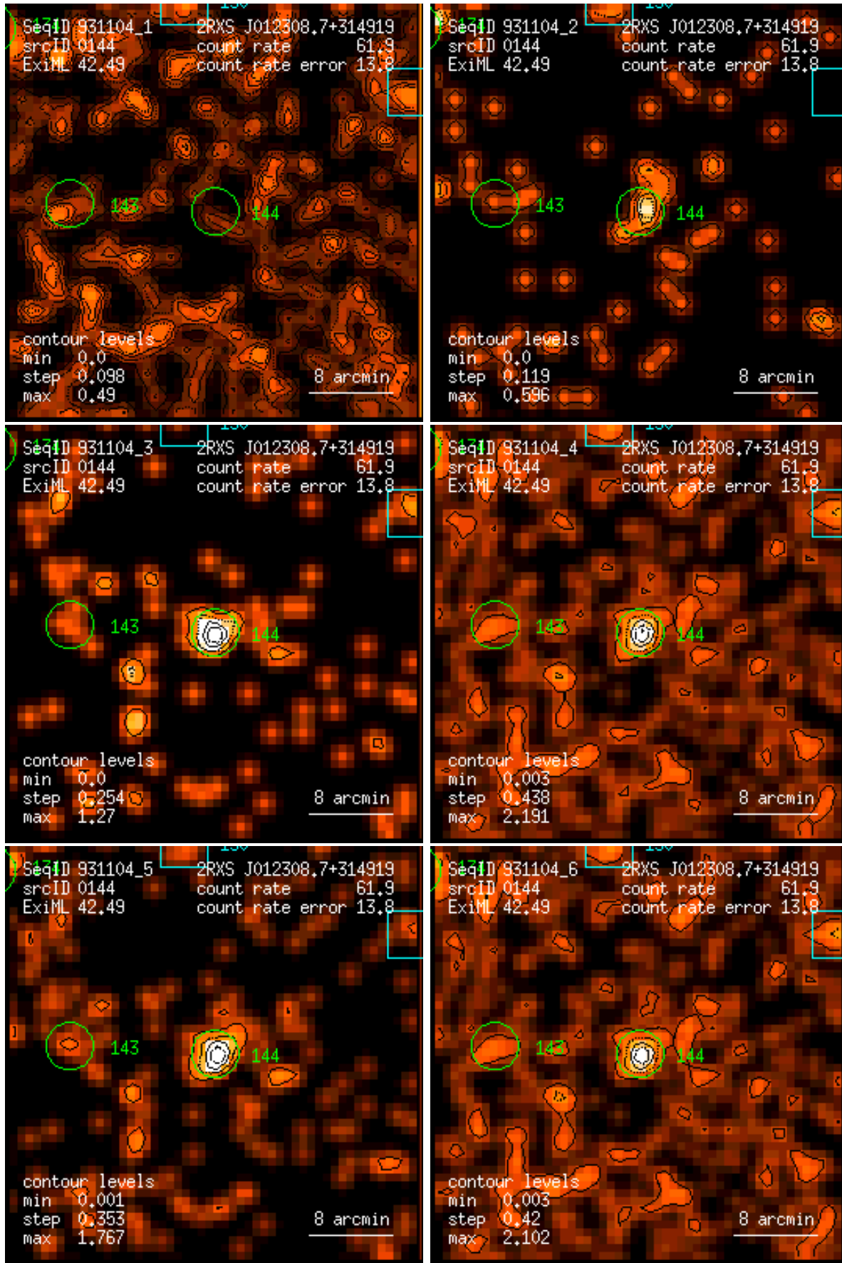
Figure 144: RASS 931104: detection 0144: band rate images, Gaussian filter: (1) PSPC channels 11 – 41, (2) 52 – 90, (3) 91 – 201, (4) 11 – 235, (5) 52 – 201, (6) 11 – 201. Broad band rates in counts/ks. Band rate contour levels in counts/ks/arcmin 2 .
