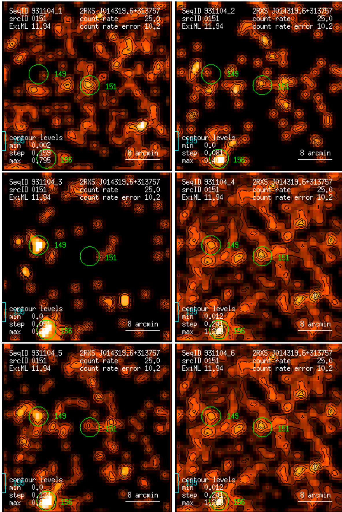
Figure 151: RASS 931104: detection 0151: band rate images, Gaussian filter: (1) PSPC channels 11 – 41, (2) 52 – 90, (3) 91 – 201, (4) 11 – 235, (5) 52 – 201, (6) 11 – 201. Broad band rates in counts/ks. Band rate contour levels in counts/ks/arcmin 2 .
