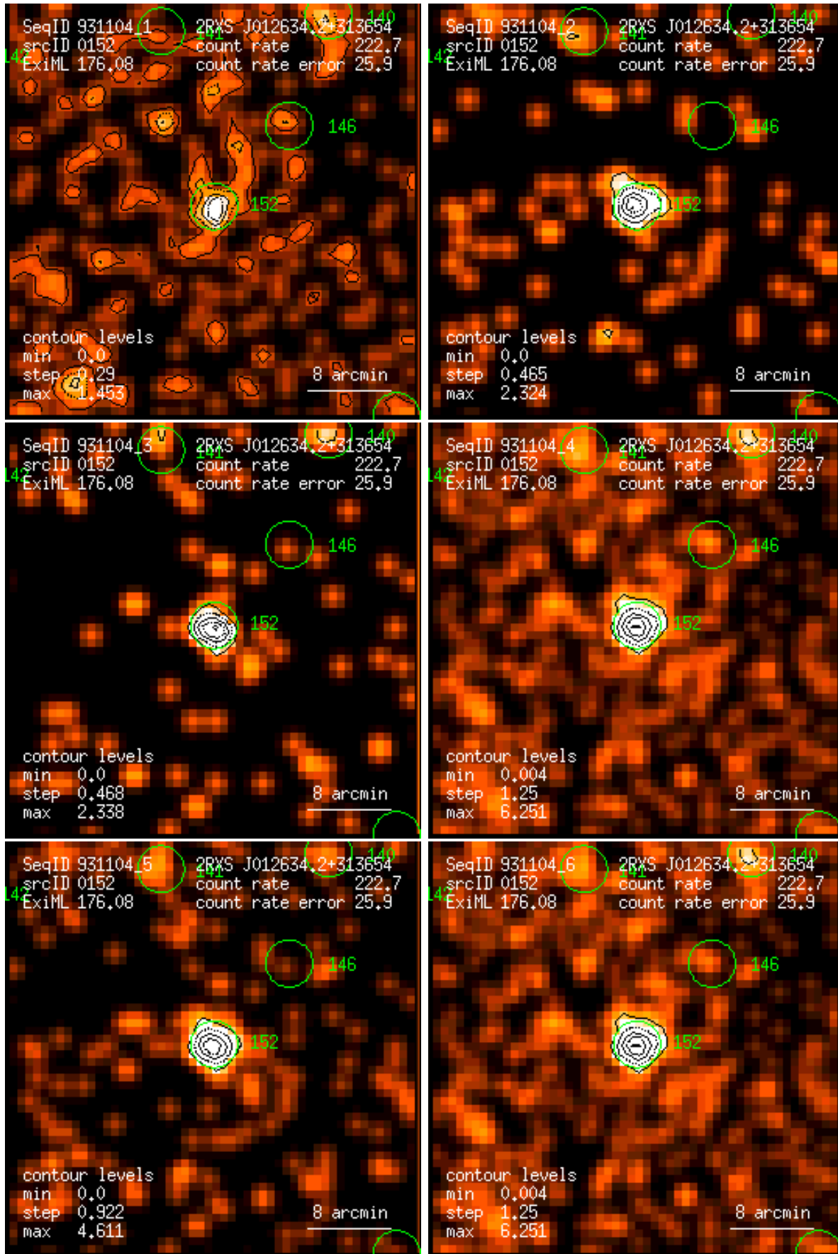
Figure 152: RASS 931104: detection 0152: band rate images, Gaussian filter: (1) PSPC channels 11 – 41, (2) 52 – 90, (3) 91 – 201, (4) 11 – 235, (5) 52 – 201, (6) 11 – 201. Broad band rates in counts/ks. Band rate contour levels in counts/ks/arcmin 2 .
