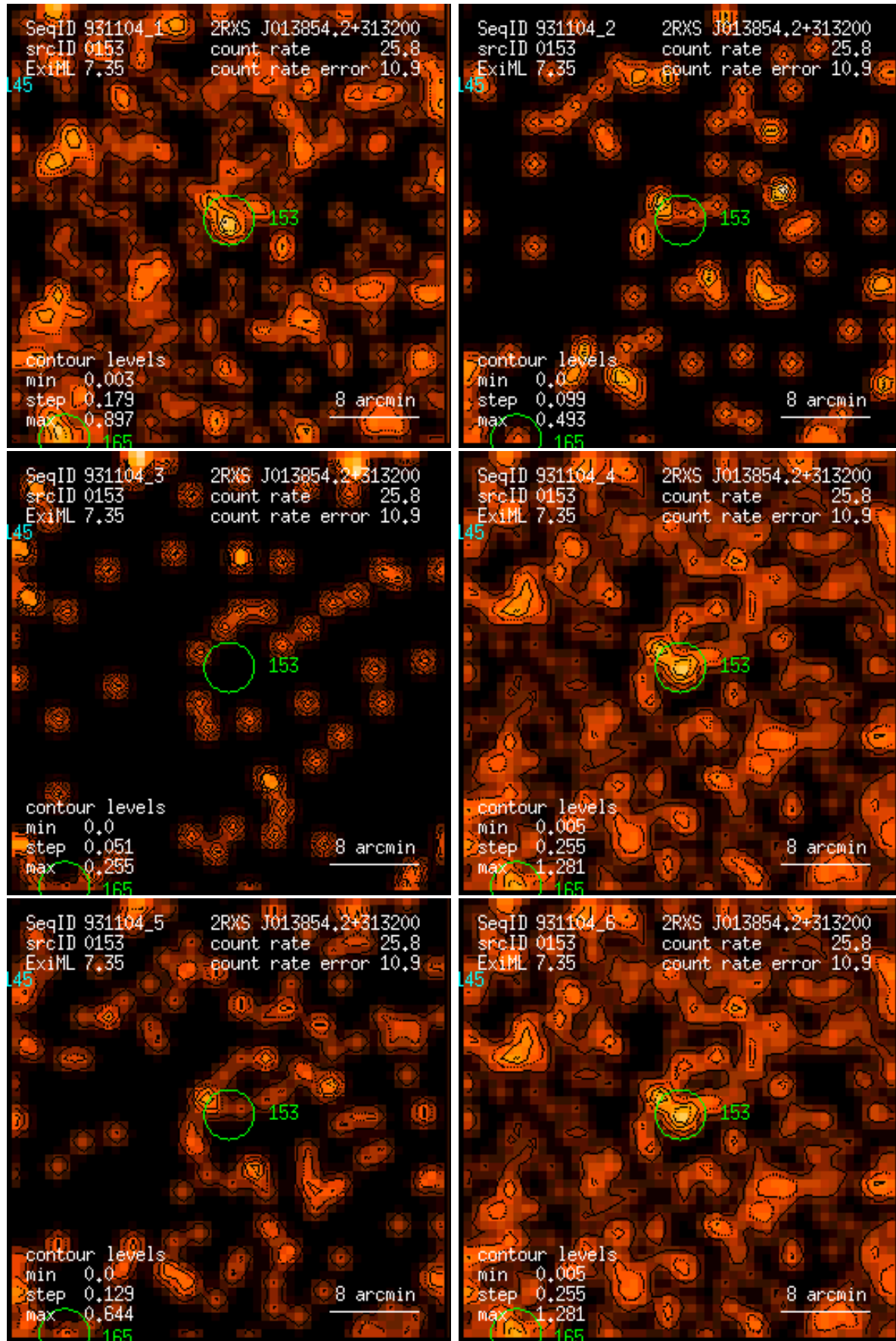
Figure 153: RASS 931104: detection 0153: band rate images, Gaussian filter: (1) PSPC channels 11 – 41, (2) 52 – 90, (3) 91 – 201, (4) 11 – 235, (5) 52 – 201, (6) 11 – 201. Broad band rates in counts/ks. Band rate contour levels in counts/ks/arcmin 2 .
