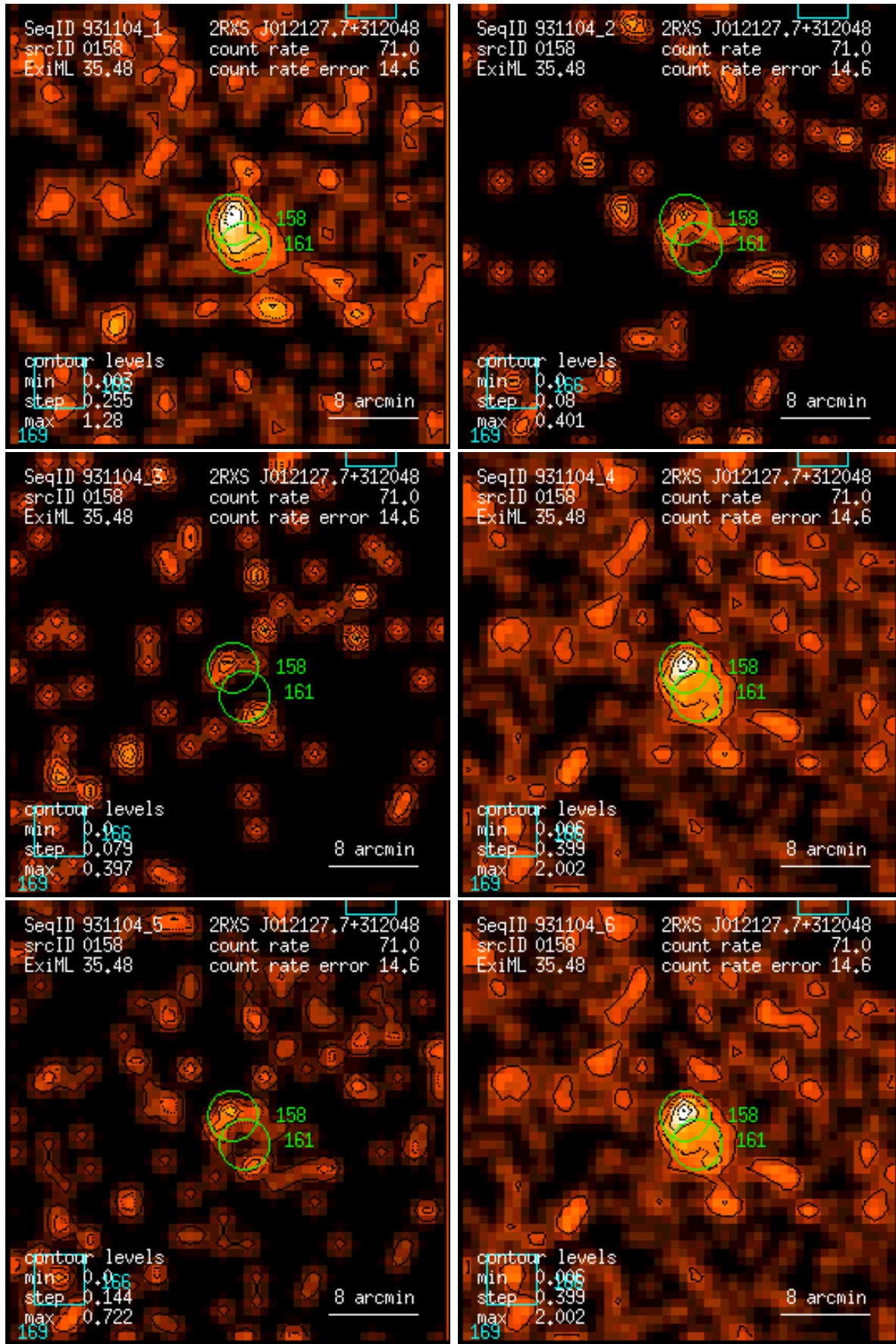
Figure 158: RASS 931104: detection 0158: band rate images, Gaussian filter: (1) PSPC channels 11 – 41, (2) 52 – 90, (3) 91 – 201, (4) 11 – 235, (5) 52 – 201, (6) 11 – 201. Broad band rates in counts/ks. Band rate contour levels in counts/ks/arcmin 2 .
