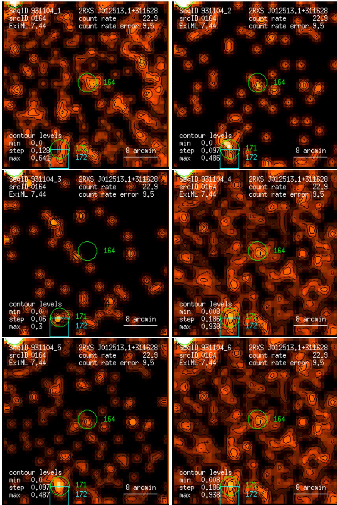
Figure 164: RASS 931104: detection 0164: band rate images, Gaussian filter: (1) PSPC channels 11 – 41, (2) 52 – 90, (3) 91 – 201, (4) 11 – 235, (5) 52 – 201, (6) 11 – 201. Broad band rates in counts/ks. Band rate contour levels in counts/ks/arcmin 2 .
