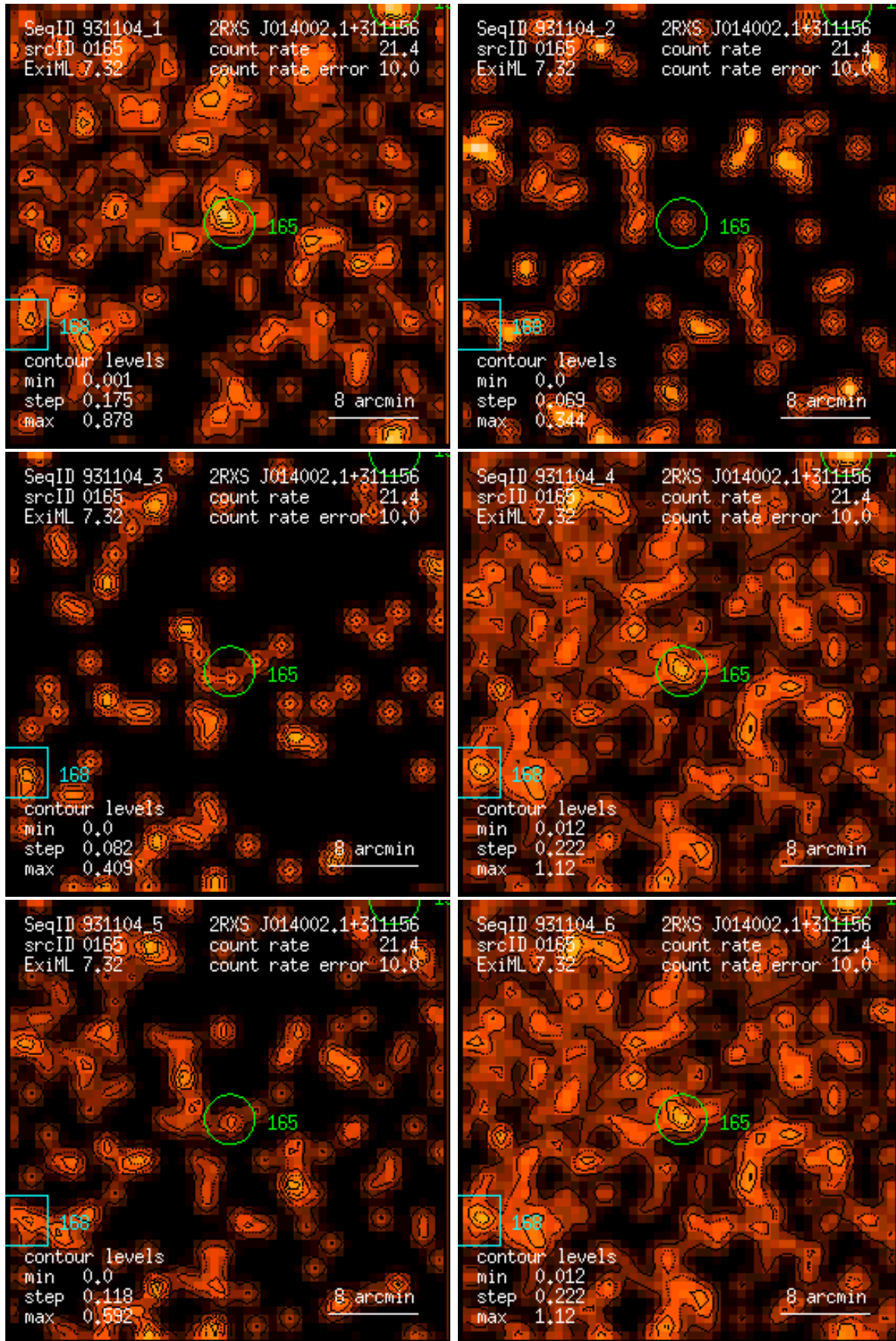
Figure 165: RASS 931104: detection 0165: band rate images, Gaussian filter: (1) PSPC channels 11 – 41, (2) 52 – 90, (3) 91 – 201, (4) 11 – 235, (5) 52 – 201, (6) 11 – 201. Broad band rates in counts/ks. Band rate contour levels in counts/ks/arcmin 2 .
