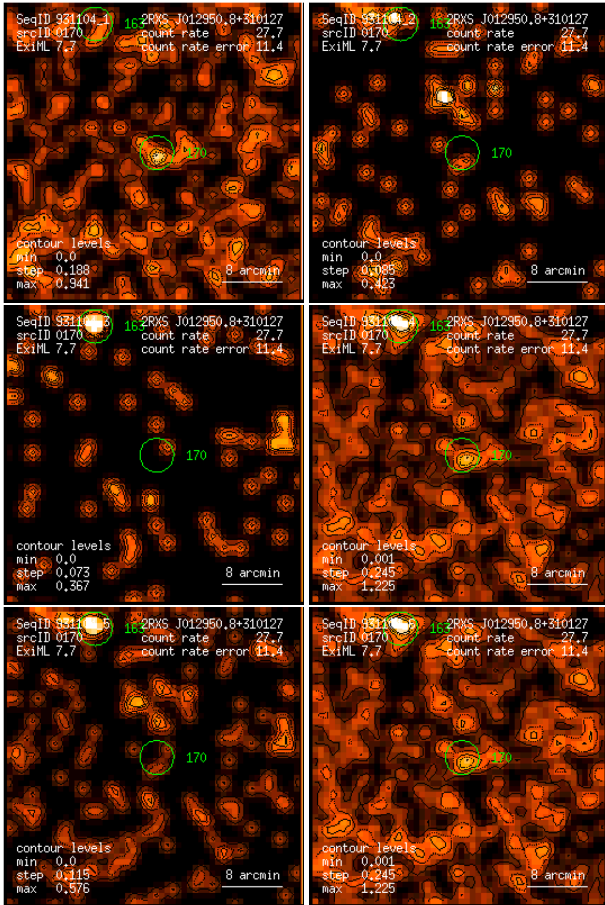
Figure 170: RASS 931104: detection 0170: band rate images, Gaussian filter: (1) PSPC channels 11 – 41, (2) 52 – 90, (3) 91 – 201, (4) 11 – 235, (5) 52 – 201, (6) 11 – 201. Broad band rates in counts/ks. Band rate contour levels in counts/ks/arcmin 2 .
