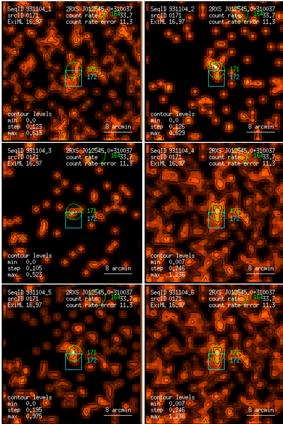
Figure 171: RASS 931104: detection 0171: band rate images, Gaussian filter: (1) PSPC channels 11 – 41, (2) 52 – 90, (3) 91 – 201, (4) 11 – 235, (5) 52 – 201, (6) 11 – 201. Broad band rates in counts/ks. Band rate contour levels in counts/ks/arcmin 2 .
