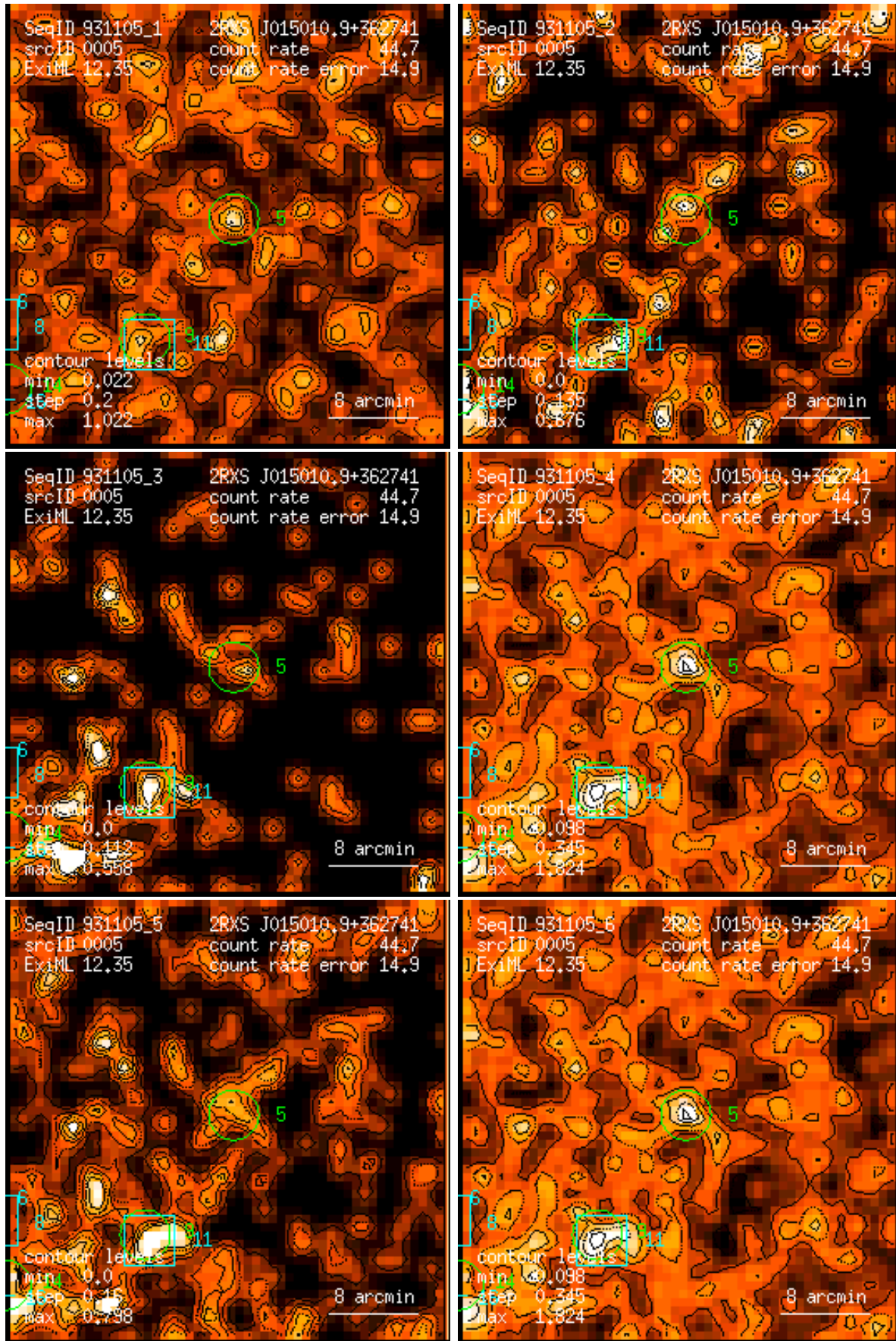
Figure 5: RASS 931105: detection 0005: band rate images, Gaussian filter: (1) PSPC channels 11 – 41, (2) 52 – 90, (3) 91 – 201, (4) 11 – 235, (5) 52 – 201, (6) 11 – 201. Broad band rates in counts/ks. Band rate contour levels in counts/ks/arcmin 2 .
