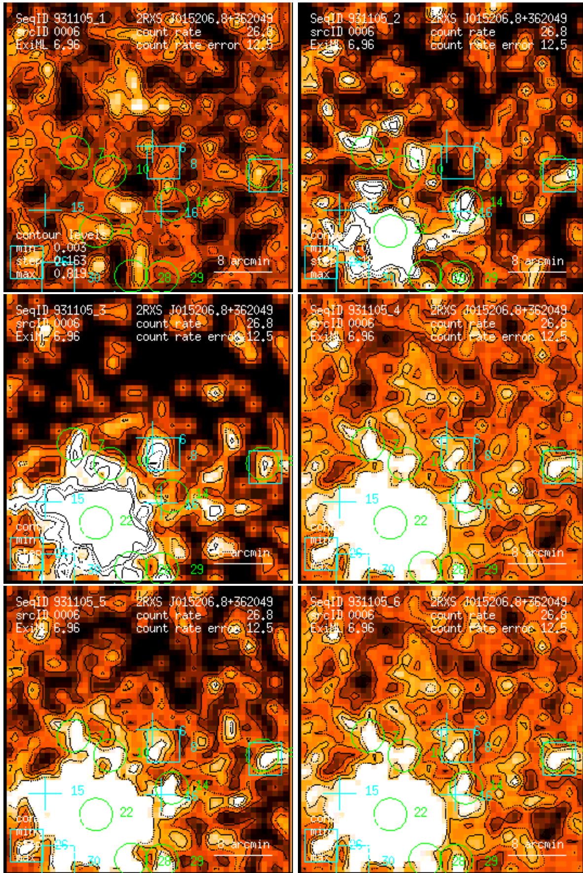
Figure 6: RASS 931105: detection 0006: band rate images, Gaussian filter: (1) PSPC channels 11 – 41, (2) 52 – 90, (3) 91 – 201, (4) 11 – 235, (5) 52 – 201, (6) 11 – 201. Broad band rates in counts/ks. Band rate contour levels in counts/ks/arcmin 2 .
